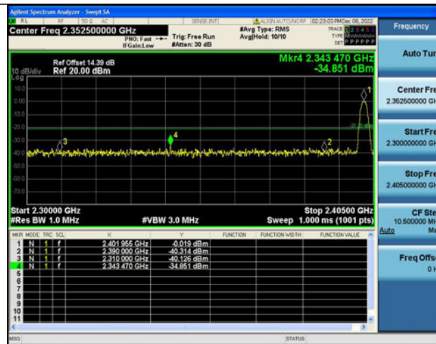
2DH5-Ant1-Low-2402-AV-2390.000
