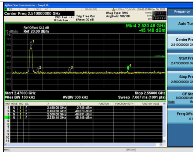
3DH5-Ant1-High-2480--1.85
