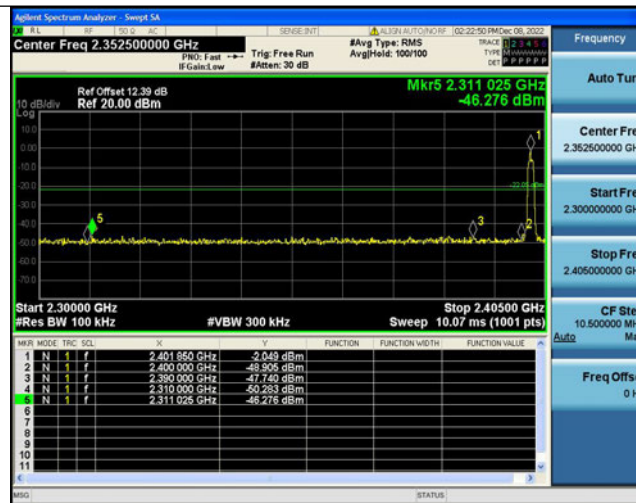
3DH5-Ant1-Low-2402--2.08
