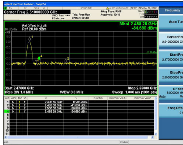
DH5-Ant1-High-2480-AV-2483.500
