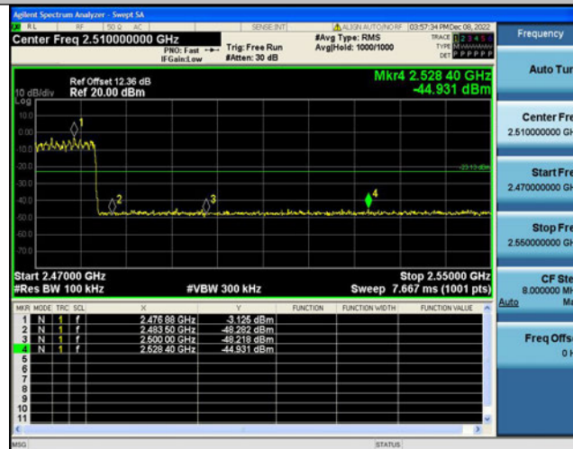
3DH5-Ant1-High-Hop_2480~3.13
