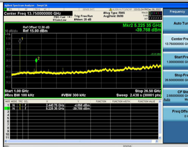
3DH5-Ant1-2441-0-Reference-5.34
