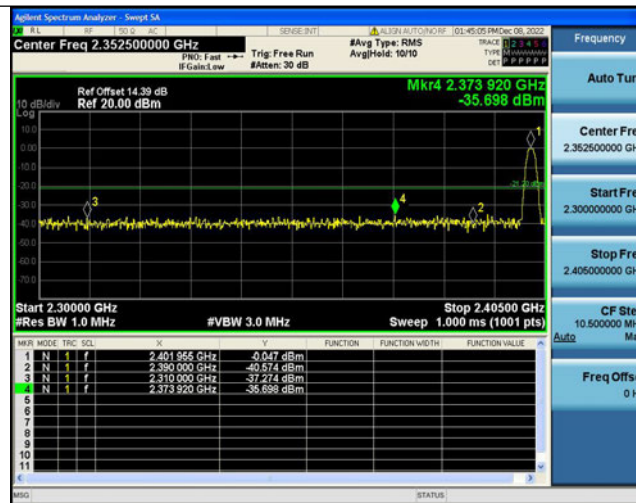
DH5-Ant1-Low-2402-AV-2390.000
