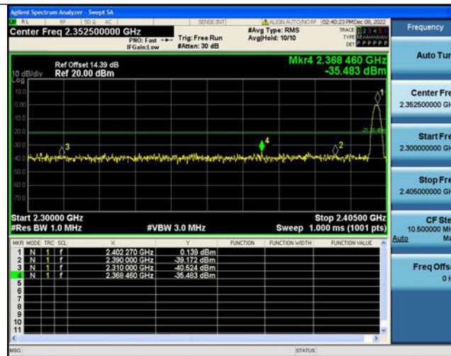
3DH5-Ant1-Low-2402-AV-2390.000
