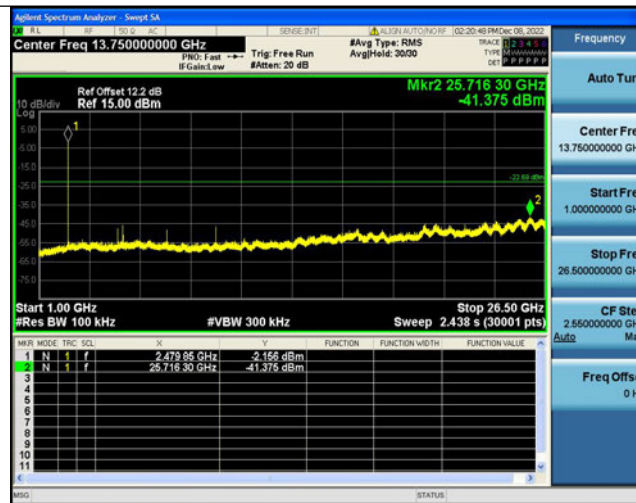
2DH5-Ant1-2402-0~Reference--5.31
