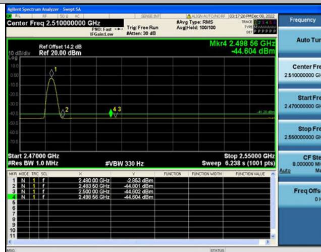
3DH5-Ant1-High-2480-Peak-2483.500
