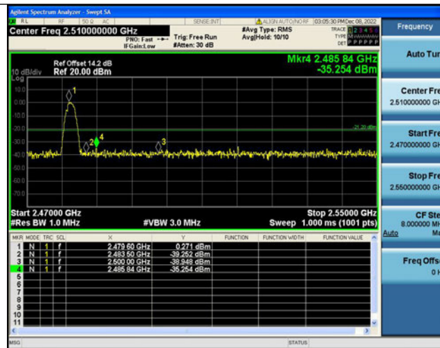
2DH5-Ant1-High-2480-AV-2483.500
