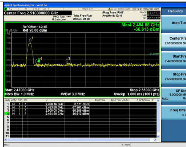
3DH5-Ant1-High-2480-AV-2483.500
