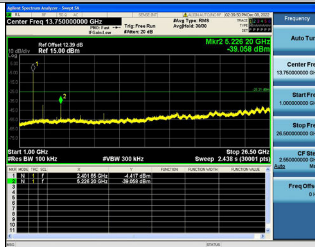
3DH5-Ant1-2402-0-Reference-5.68
