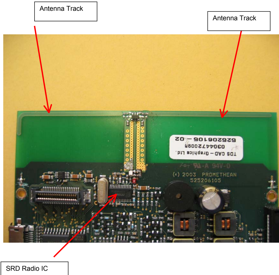
ActivBoard PCB – SRD Antenna Locations
