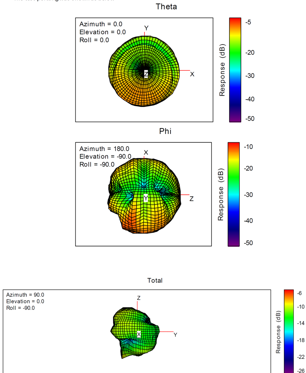
3D RDA5875Y Antenna Gain Free Space-2402MHz
