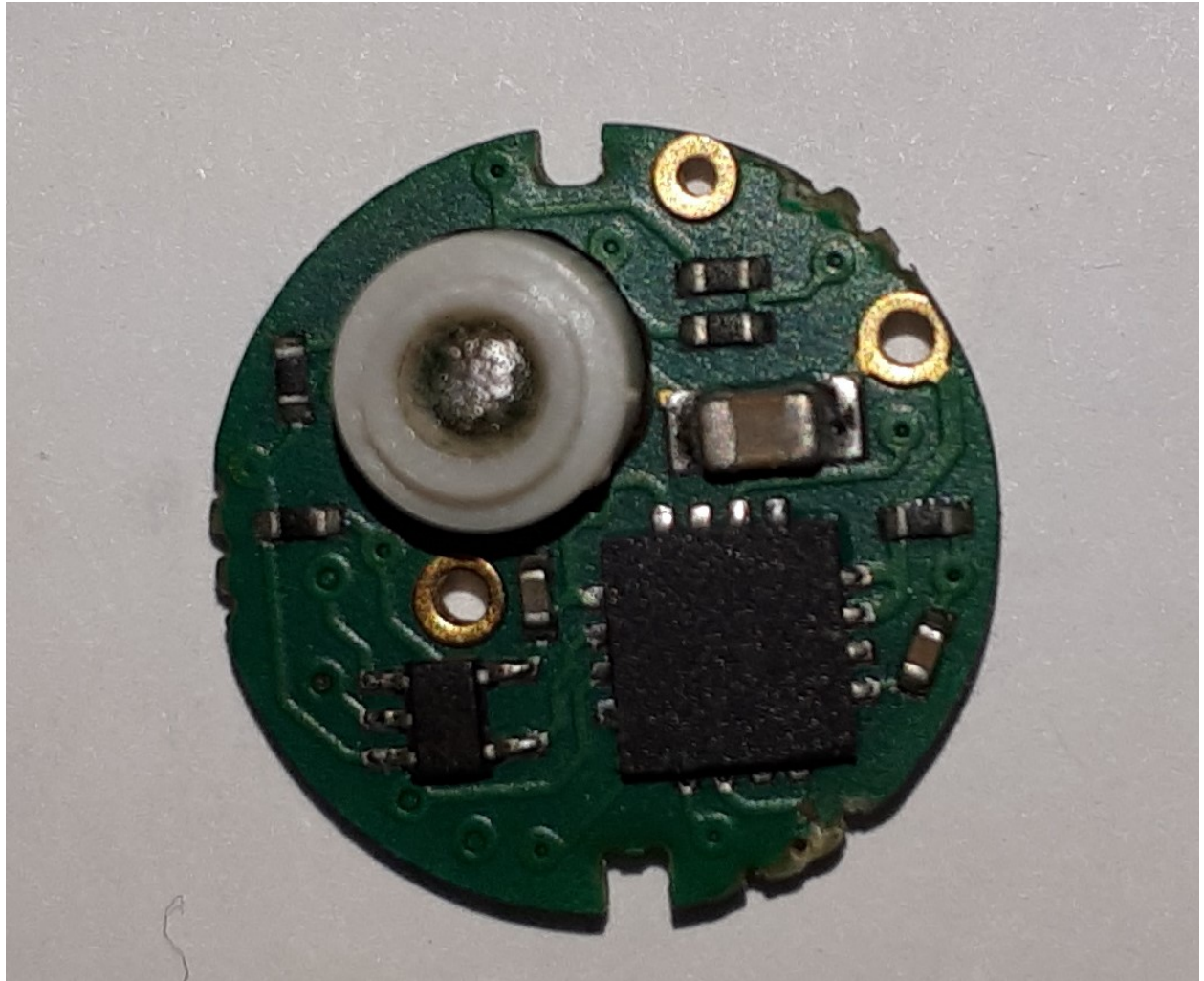
Figure 1: PCB Top View
