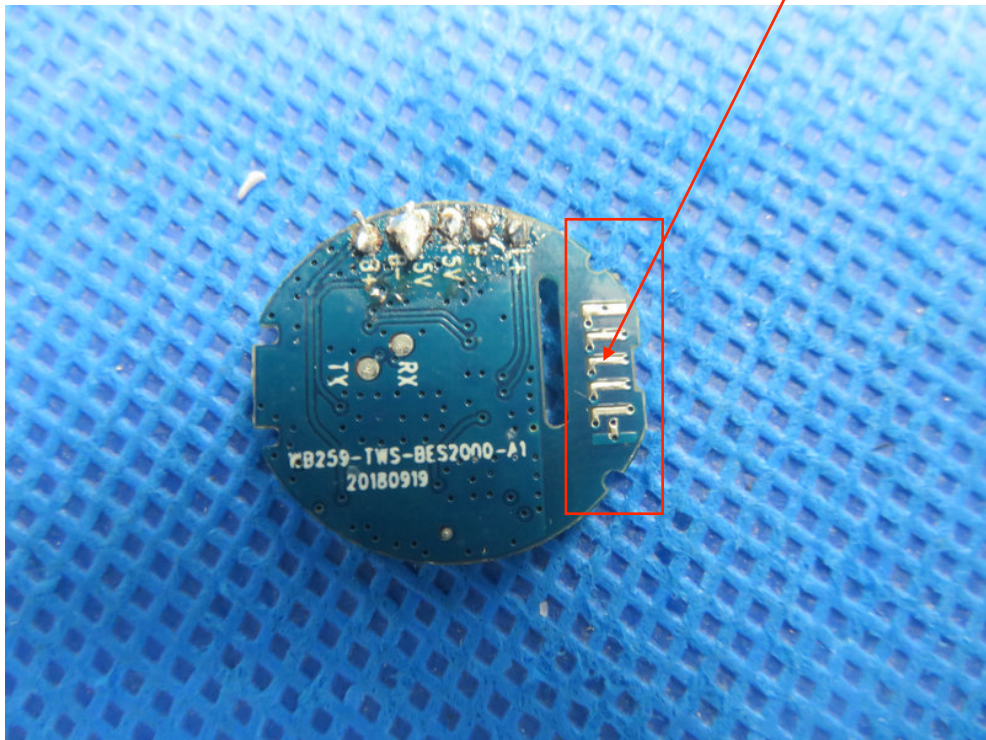
BT Antenna
