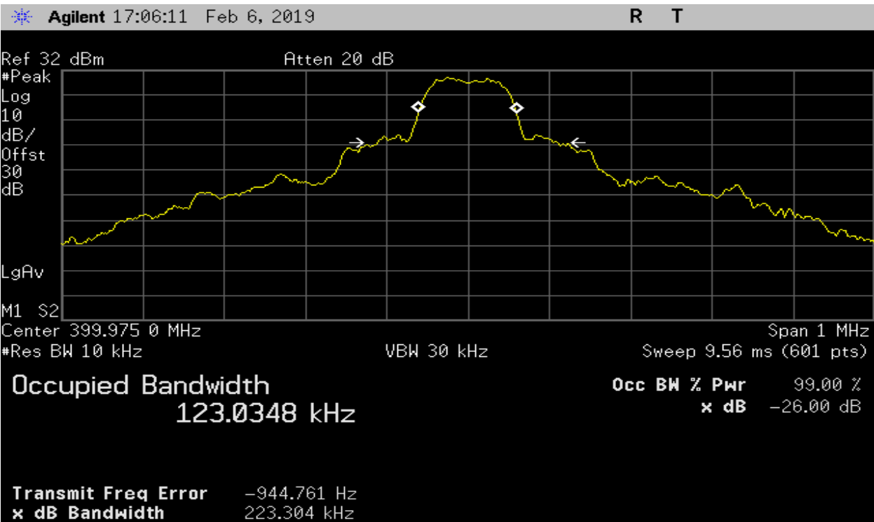
Plot 3 – Low Channel – 26dB Bandwidth
