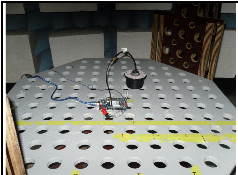
Test Setup Photo # 7 (Black Antenna)
