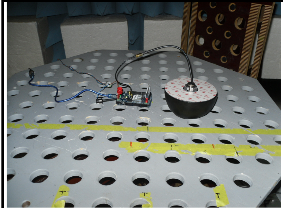
Test Setup Photo # 6 (Grizzly Antenna)
