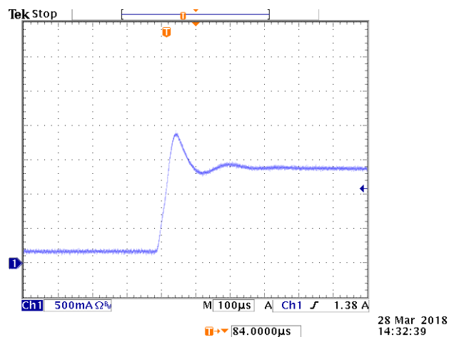
Figure 3: Hiberband modem transmitter current consumption (continuous wave)
