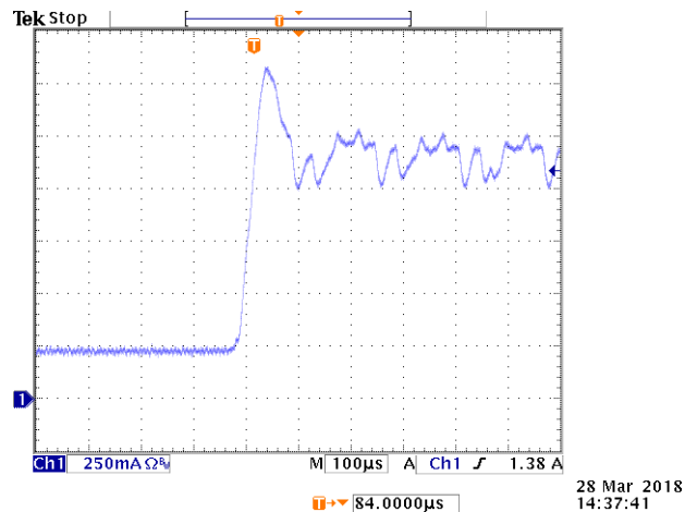
Figure 2: Hiberband transmission burst current consumption
