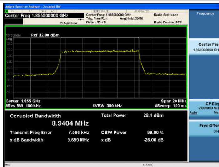
Band2-10MHz-16QAM-18650-50RB#0-8.9404
