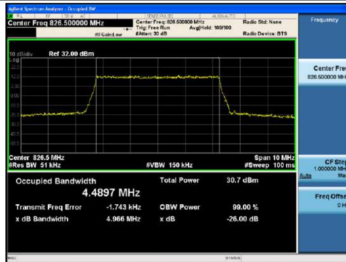
Band5-5MHz-QPSK-20425-25RB#0-4.4897
