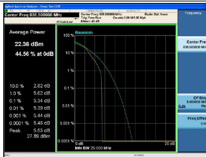
Band5-10MHz-16QAM-20525-1RB#0
