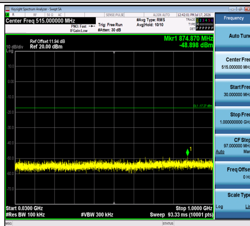
2DH5-Ant1-2441-30~1000-PASS
