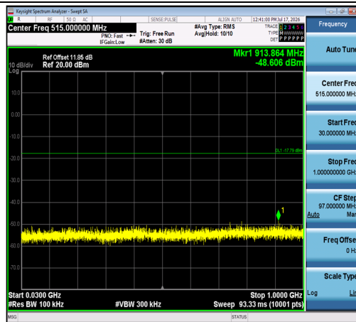
2DH5-Ant1-2402-30~1000-PASS
