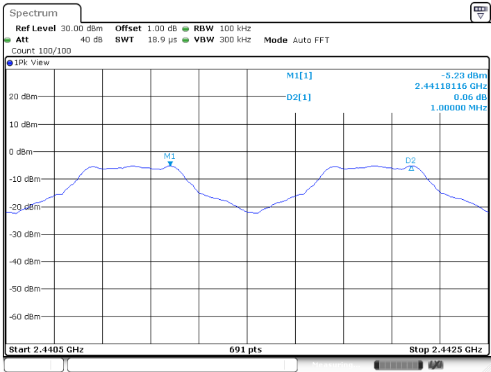
GFSK Modulation
