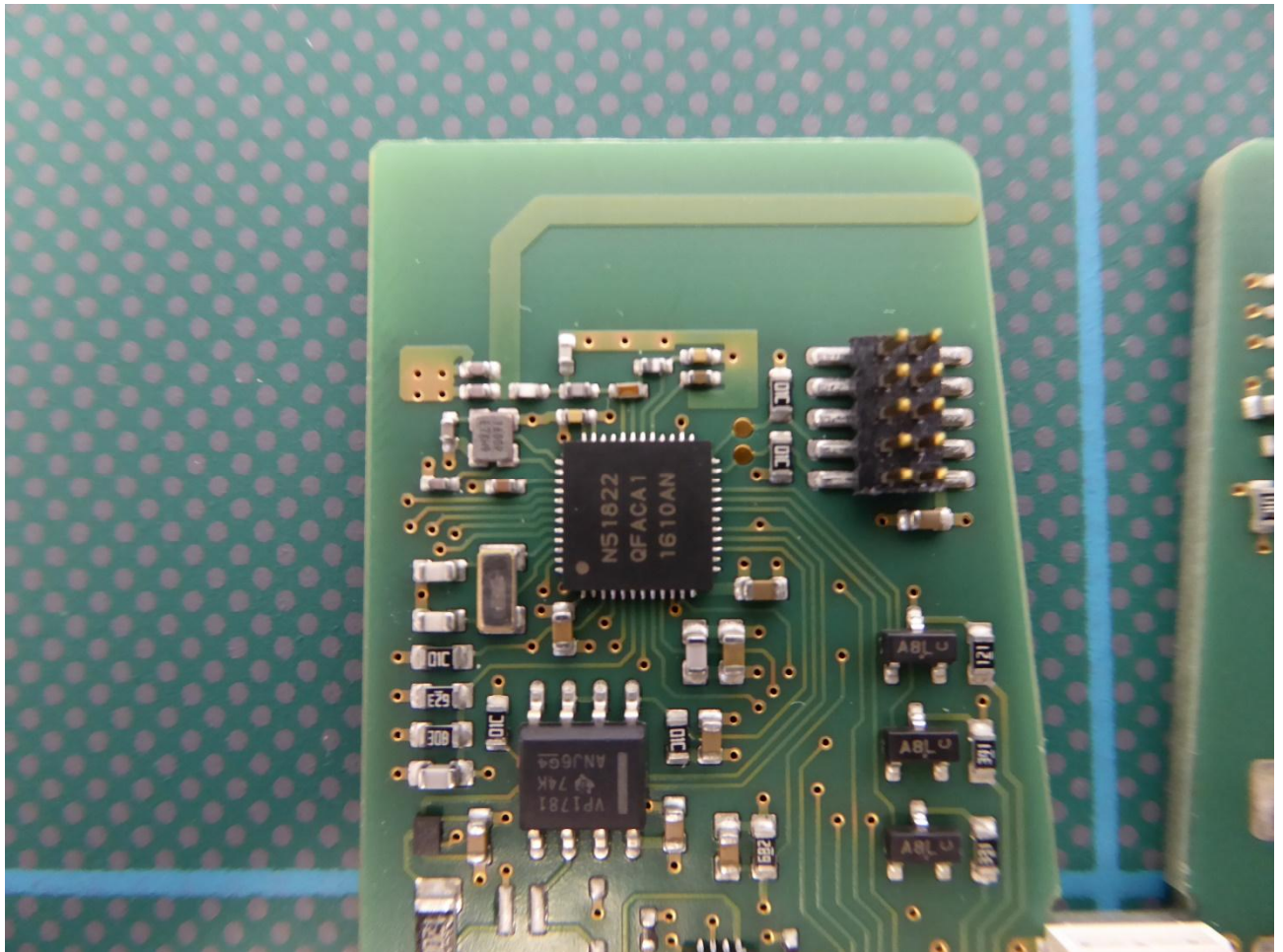
EUT – radio chip and antenna – detail view
