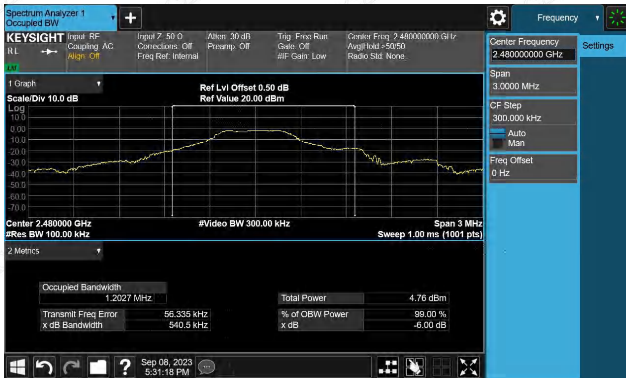
Figure 12: The plots of 99% Bandwidth, BLE-1Mbps, 2480MHz
