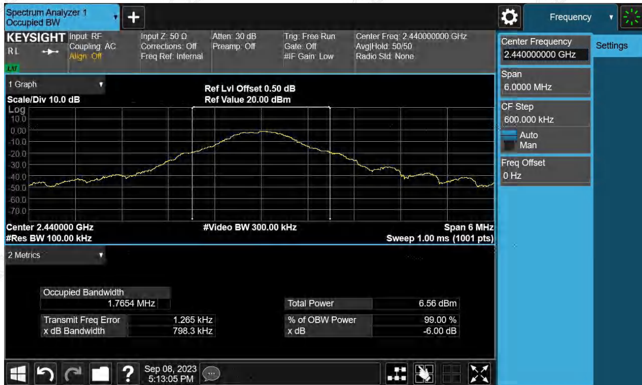
Figure 16: The plots of 99% Bandwidth, BLE-2Mbps, 2440MHz
