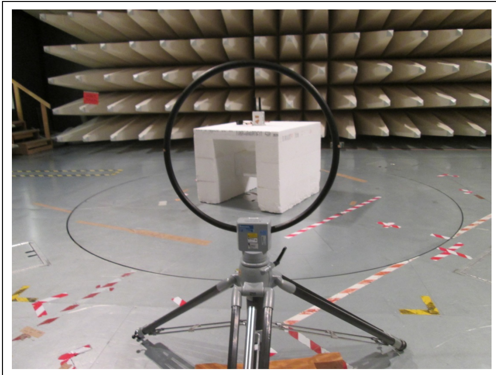
Photograph A1-1: Radiated emissions 9 kHz – 30 MHz at 3 m distance
