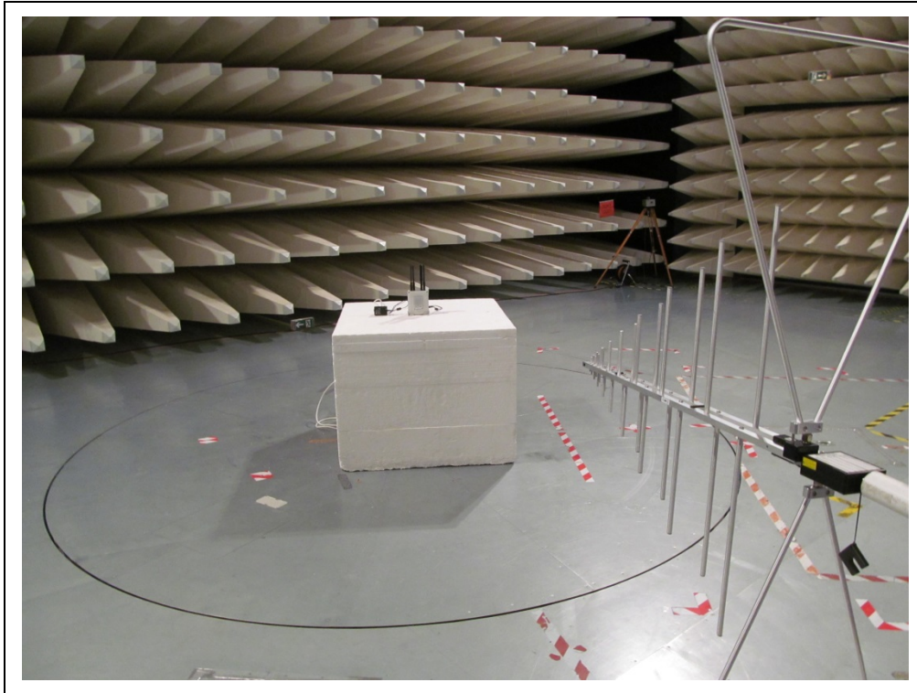
Photograph A1-1: Radiated emissions 30 – 1000 MHz at 3 m distance
