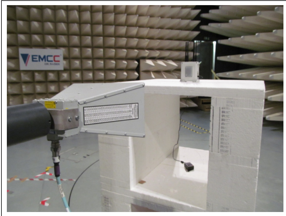
Photograph A1-3: Radiated emissions 6 – 18 GHz at 1 m distance
