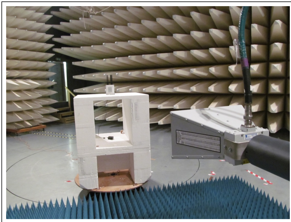
Photograph A1-2: Radiated emissions 1 – 6 GHz at 3 m distance
