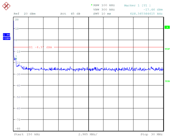
Diagram 18: conducted spurious emissions of channel 3 (carrier)
