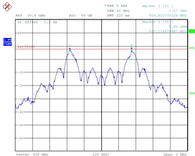
Diagram 10: PSD of channel 1
