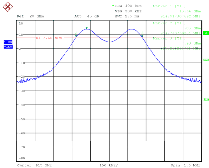
Diagram 4: 6 dB bandwidth of channel 1
