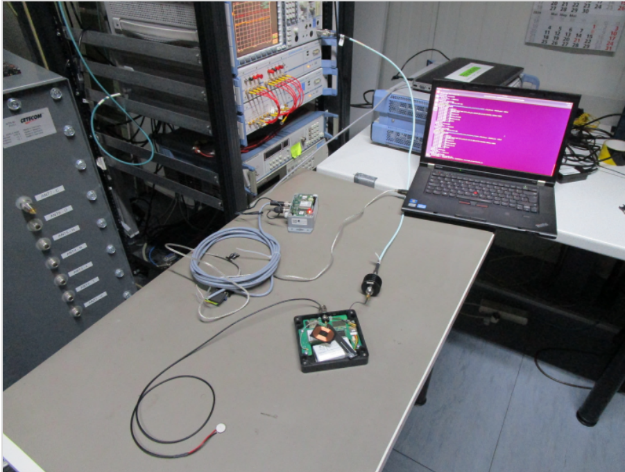
Photograph 5: EUT Test Setup conducted Measurements in the radio lab
