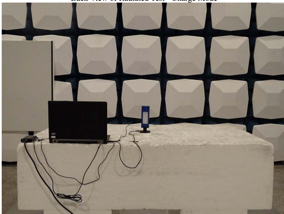
Back View of Radiated Test - Charge Mode
