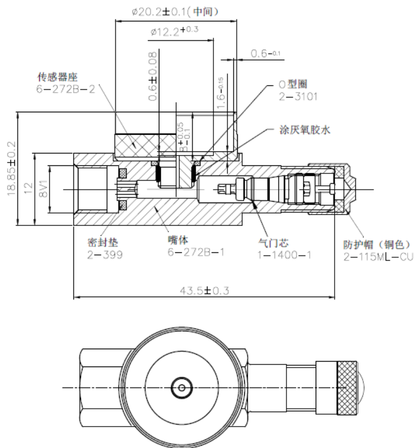
Fig. 1 - Metallic external shell, cross section and view from above (VEX1712S1, VEX1712S2, VEX1712SPH1)
