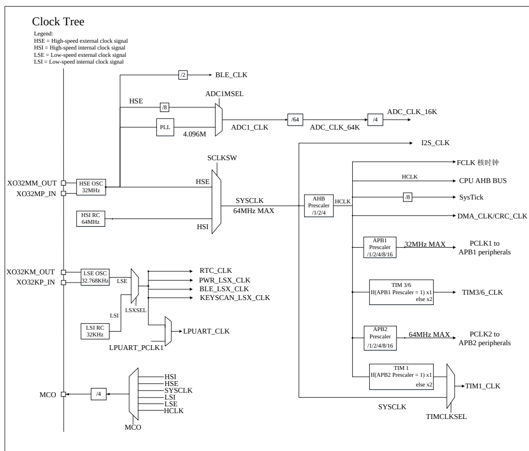
Figure 2-2 Clock Tree
