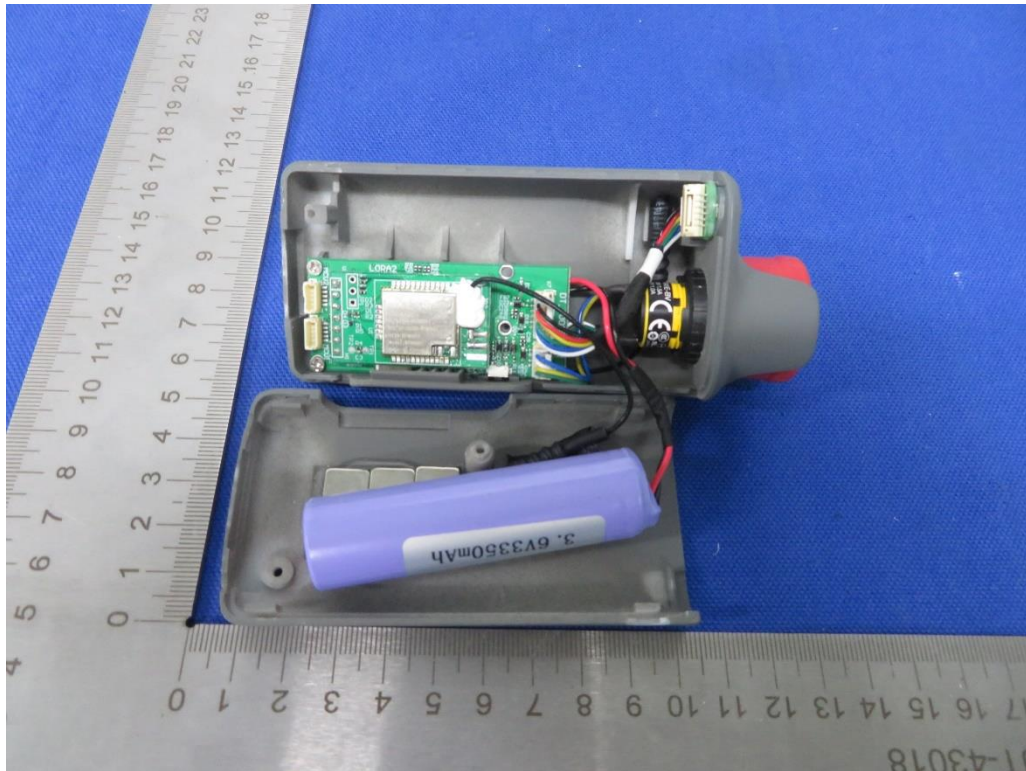
The Host Wireless Emergency-stop
