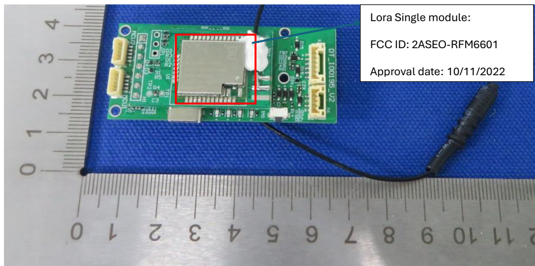
Lora Single module: FCC ID: 2ASEO-RFM6601
