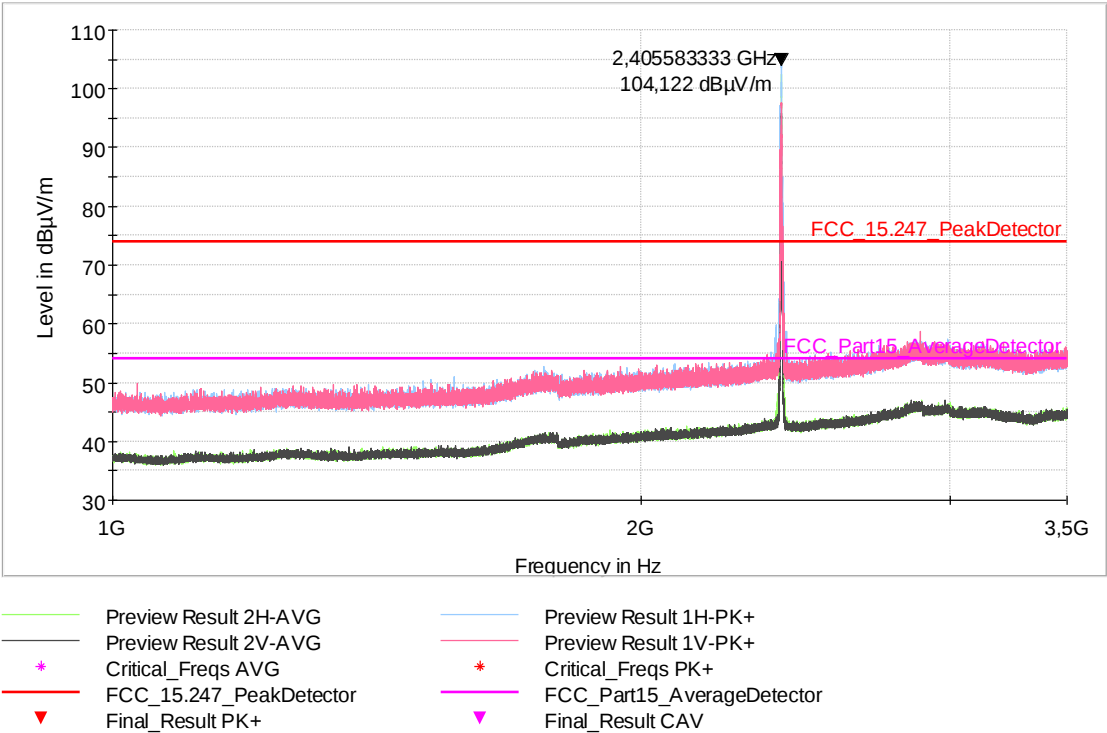
Fig. 34: Sample #1. Mode 1. Frequency range: 1 GHz – 3.5 GHz. Channel Low
