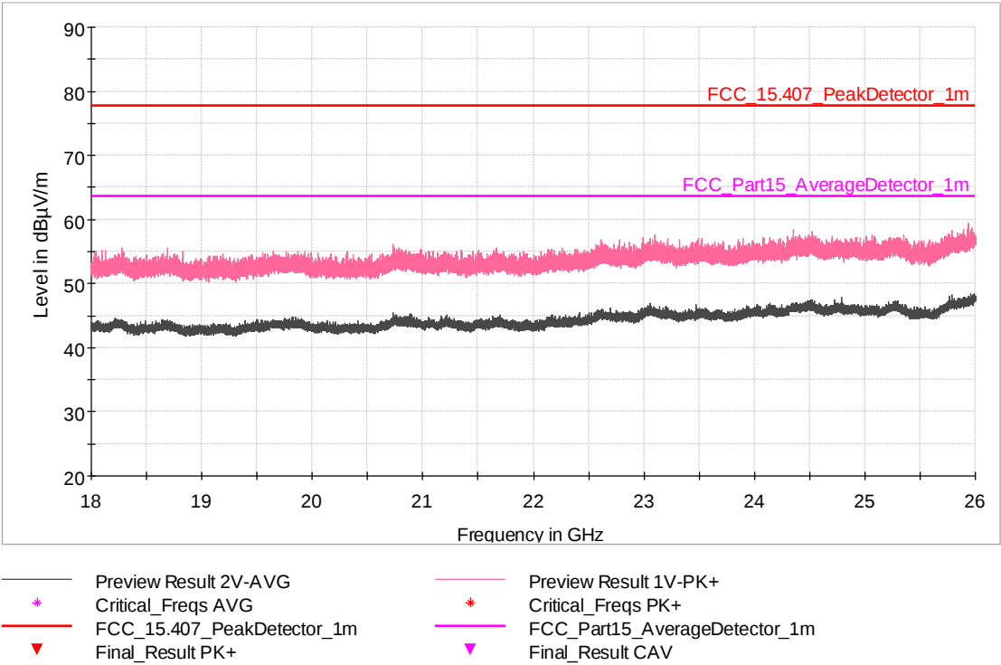
Fig. 41: Sample #1. Mode 1. Frequency range: 18 GHz – 26 GHz. Channel Middle
