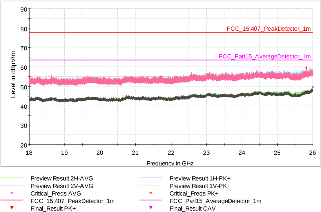
Fig. 42: Sample #1. Mode 1. Frequency range: 18 GHz – 26 GHz. Channel High
