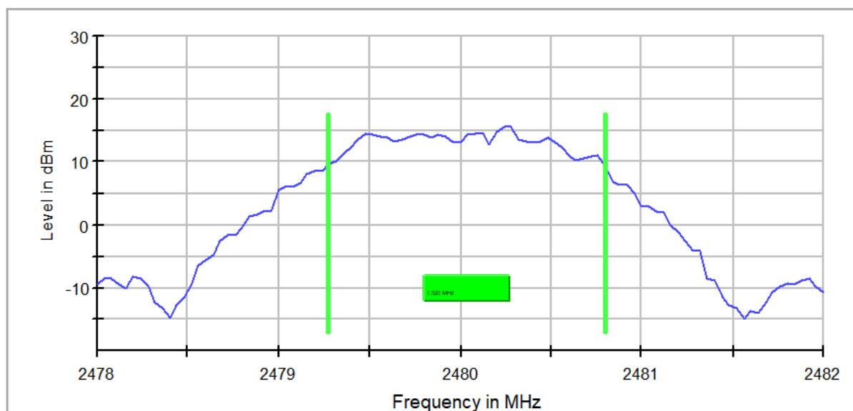
Fig. 7: Channel High - DTS Bandwidth
