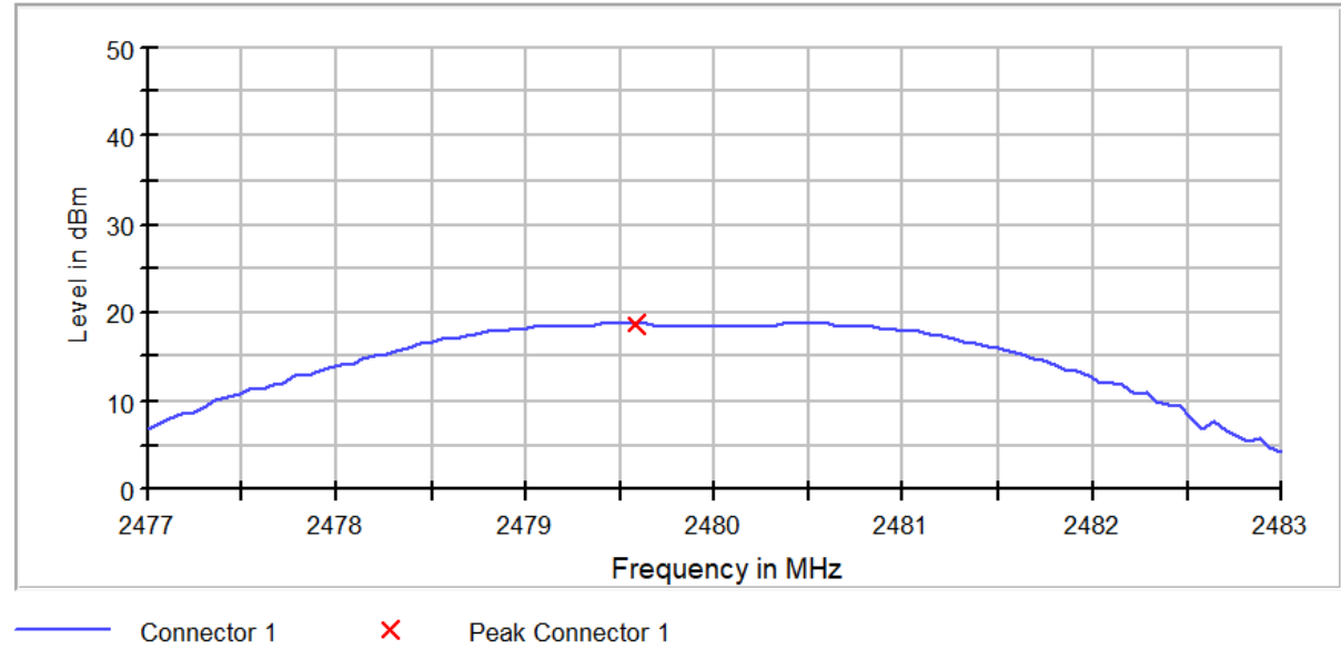
Fig. 11: Channel High - Maximum Peak Conducted Output Power
