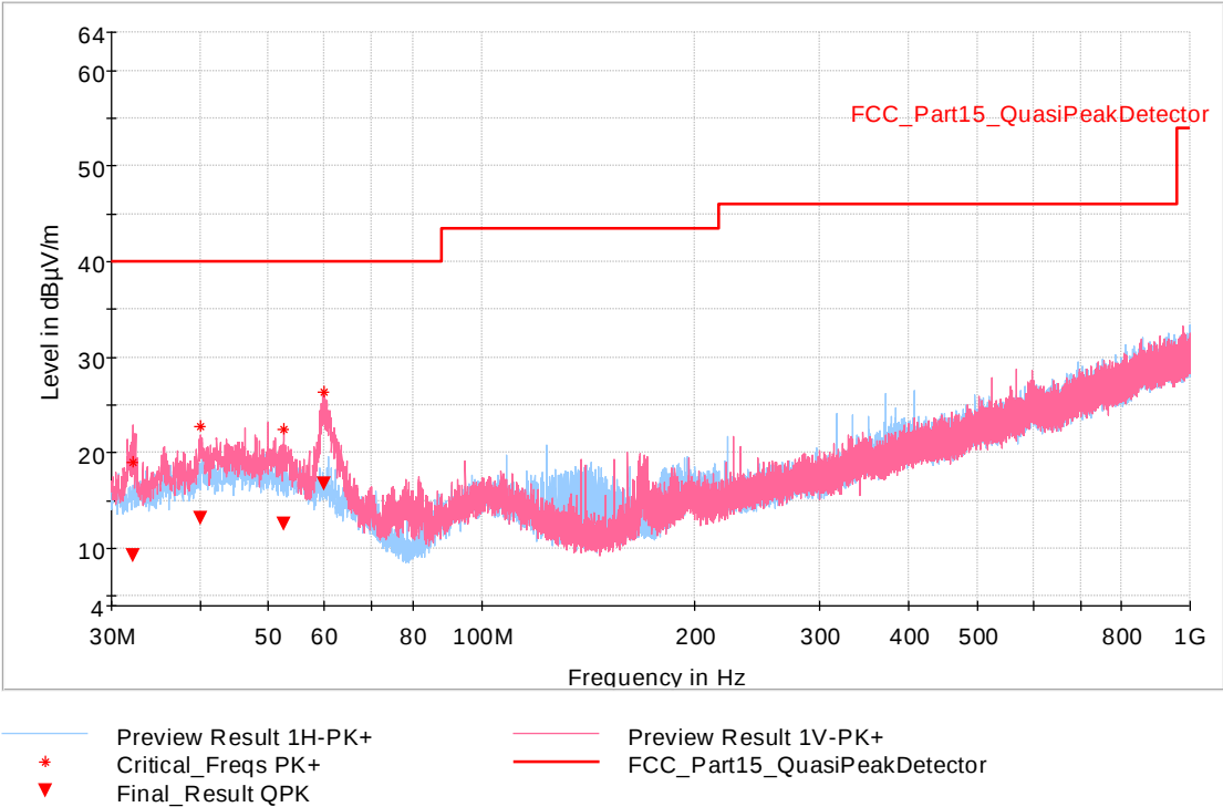
Fig. 31: Sample #1. Mode 1. Frequency range: 30 MHz – 1 GHz. Channel Low
