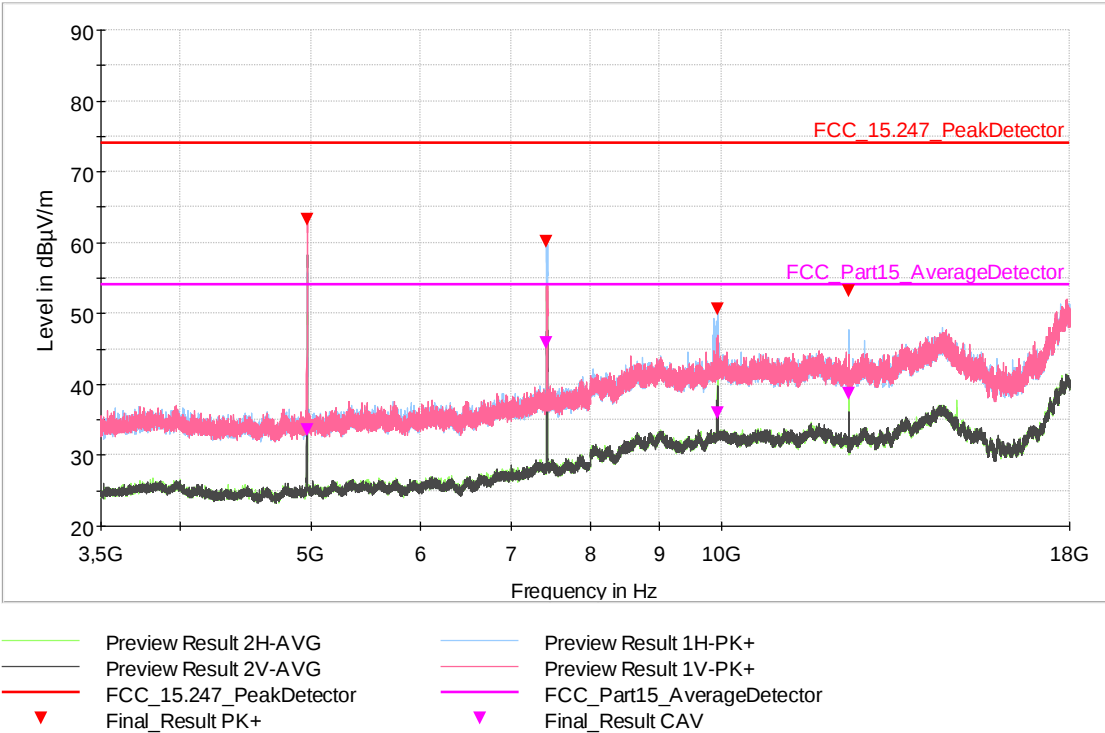
Fig. 38: Sample #1. Mode 1. Frequency range: 3.5 GHz – 18 GHz. Channel Middle
