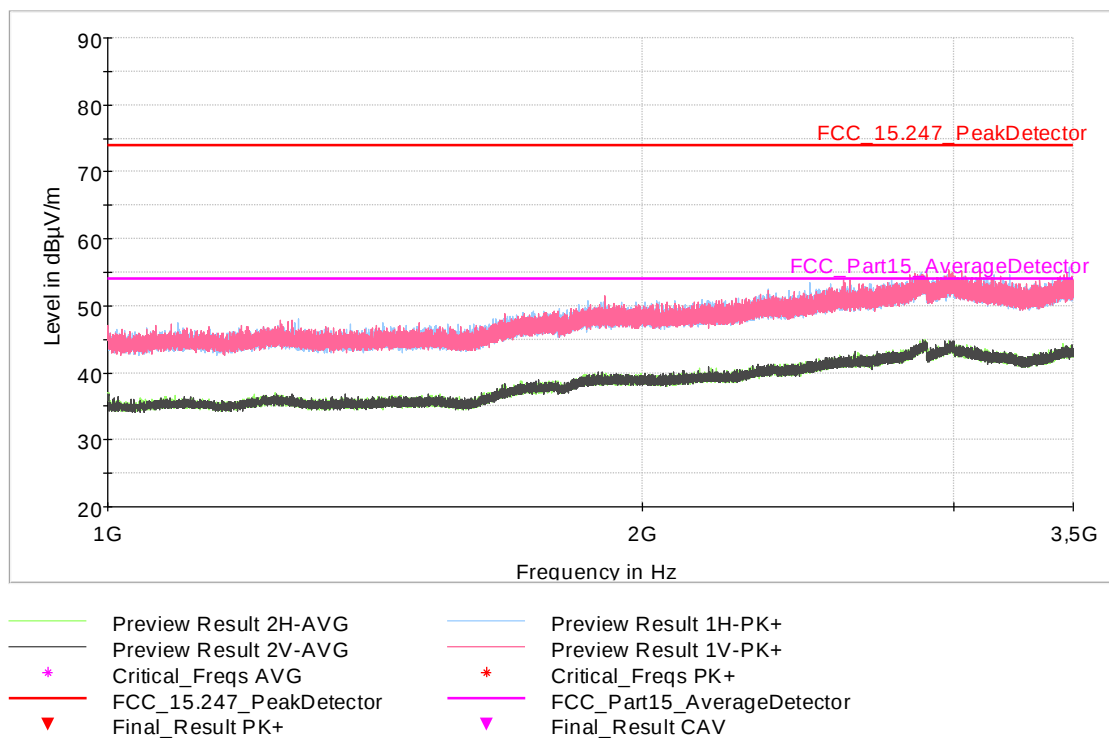
Fig. 28: Ambient level. Frequency range: 1 GHz – 3.5 GHz
