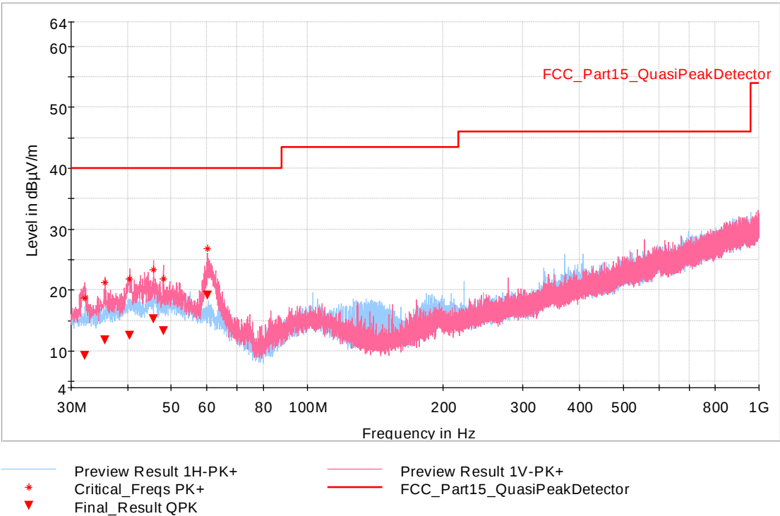
Fig. 32: Sample #1. Mode 1. Frequency range: 30 MHz – 1 GHz. Channel Middle
