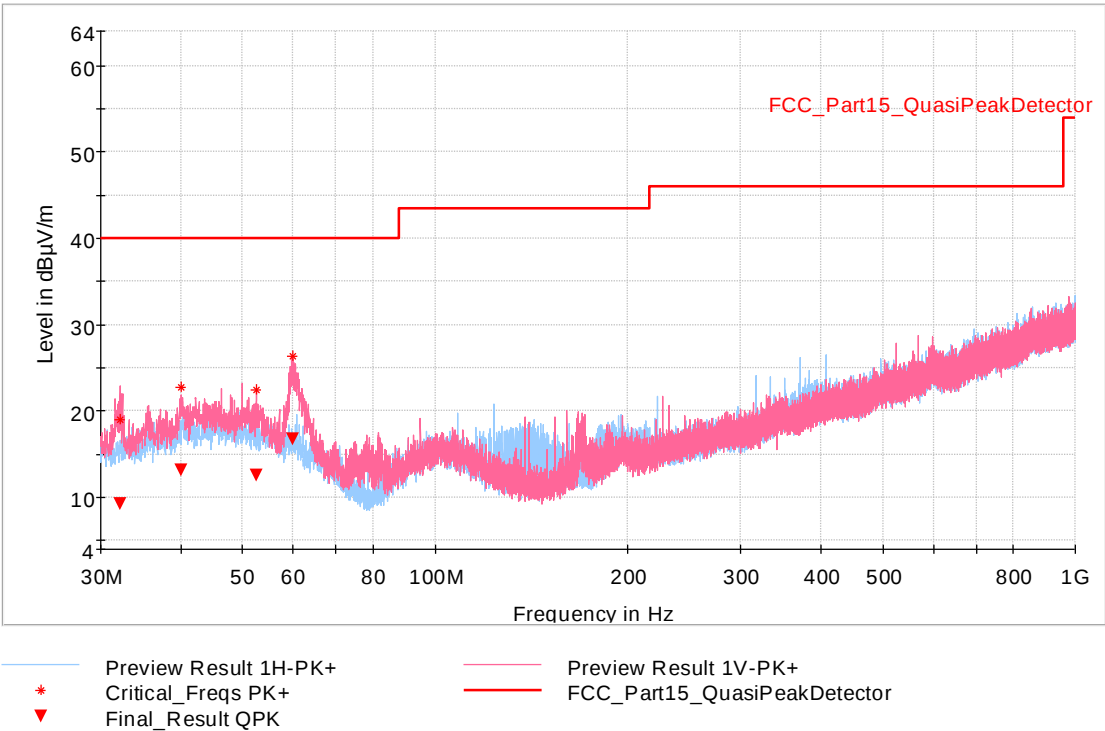
Fig. 33: Sample #1. Mode 1. Frequency range: 30 MHz – 1 GHz. Channel High
