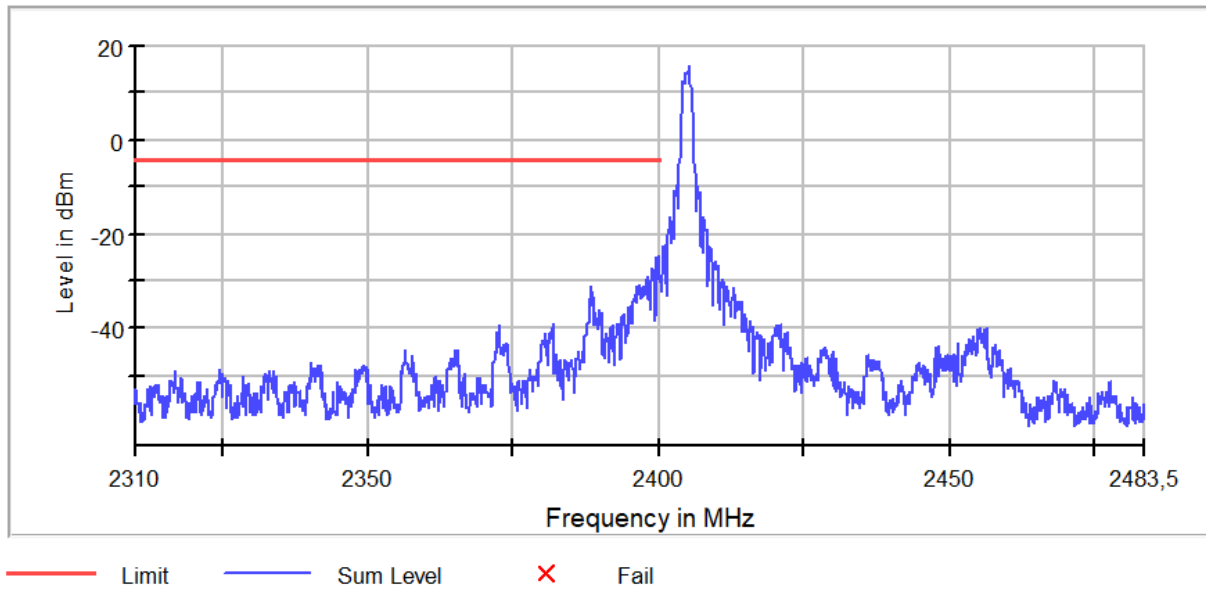
Fig. 17: Channel - Low Band Edge
