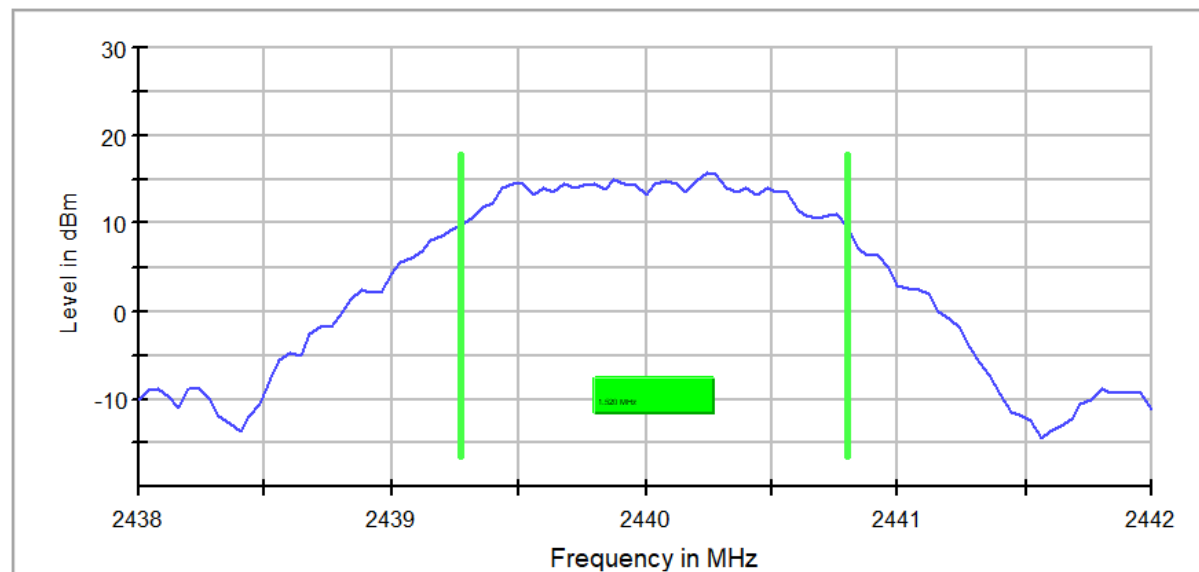
Fig. 6: Channel Middle -DTS Bandwidth
