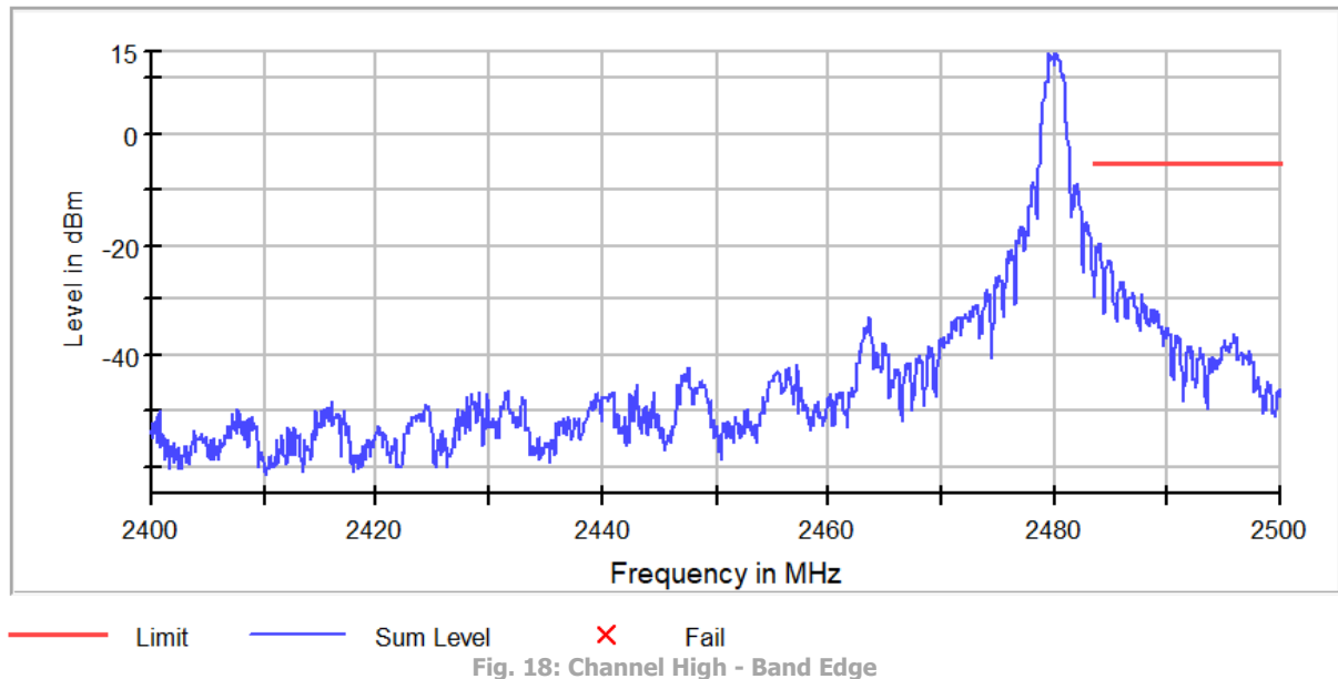
Fig. 18: Channel High - Band Edge
