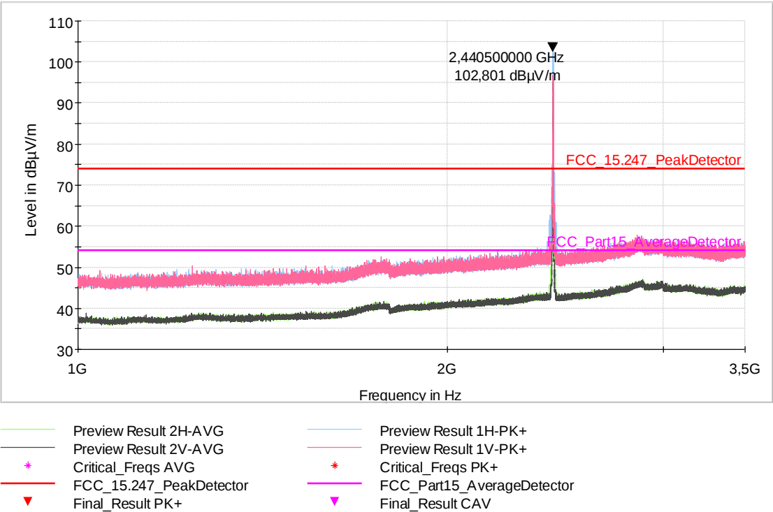
Fig. 35: Sample #1. Mode 1. Frequency range: 1 GHz – 3.5 GHz. Channel Middle
