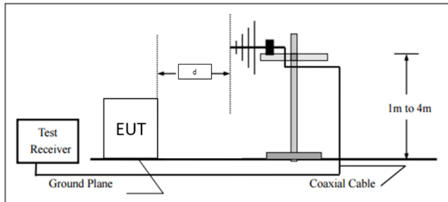
Fig. 25: Radio-frequency radiated emissions of floor-standing setup equipment from 30 MHz to 1000 MHz
