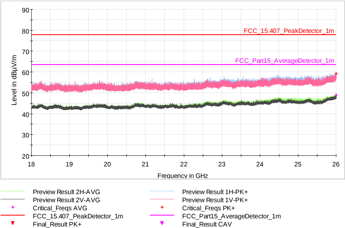
Fig. 40: Sample #1. Mode 1. Frequency range: 18 GHz – 26 GHz. Channel Low
