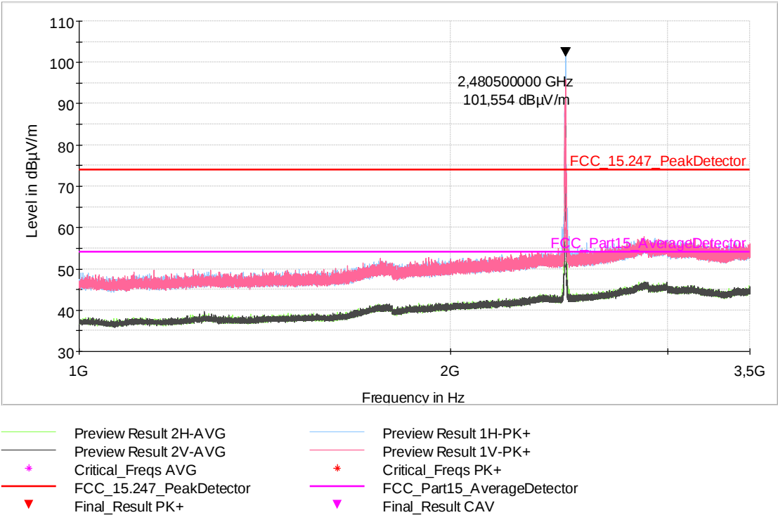
Fig. 36: Sample #1. Mode 1. Frequency range: 1 GHz – 3.5 GHz. Channel High
