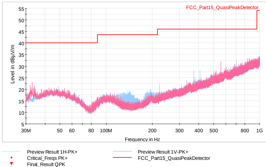
Fig. 27: Ambient level. Frequency range: 30 MHz – 1 GHz
