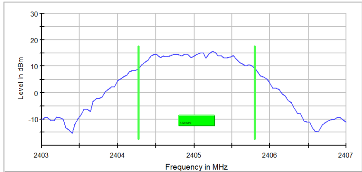
Fig. 5: Channel Low - DTS Bandwidth
