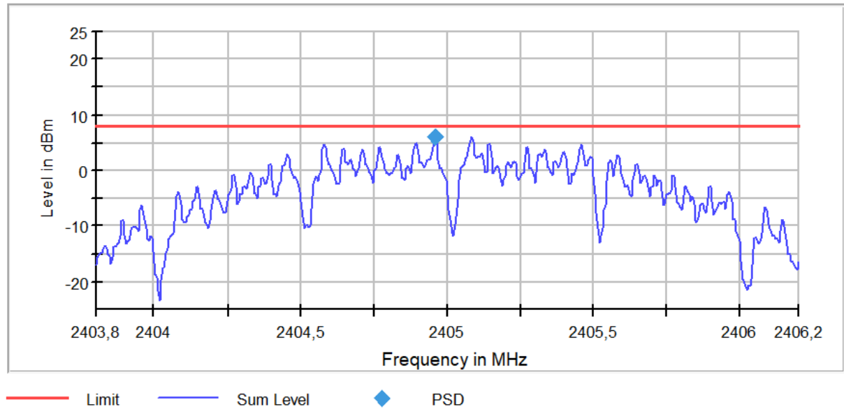
Fig. 14: Channel Low - Power Spectral Density
