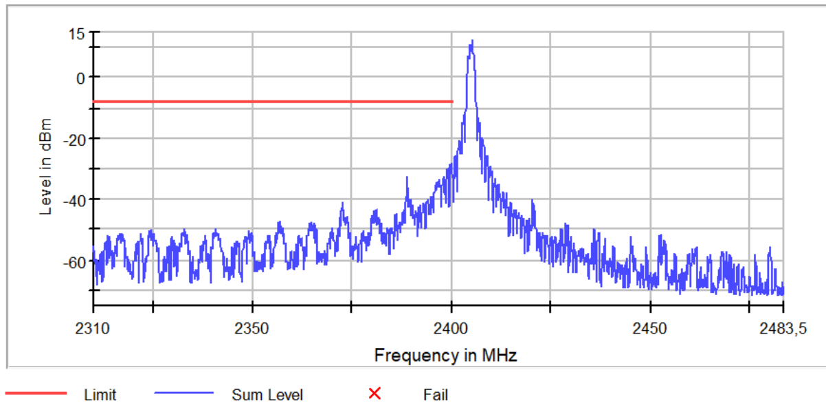
Fig. 18: Channel - Low Band Edge
