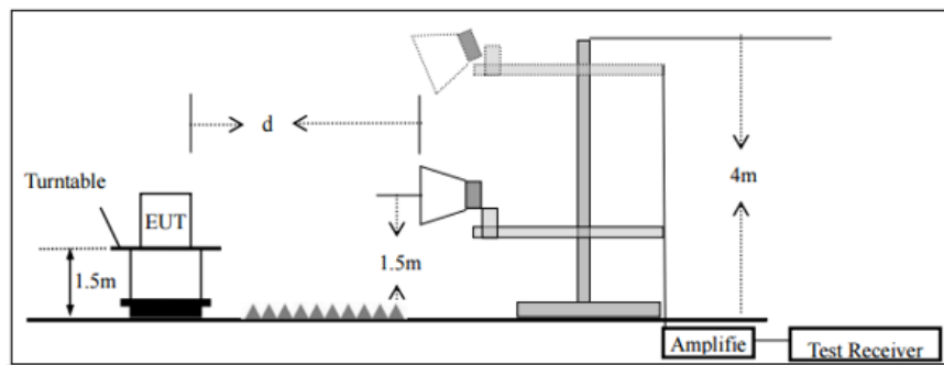
Fig. 22: Radio-frequency radiated emissions setup of table top equipment above 1 GHz
