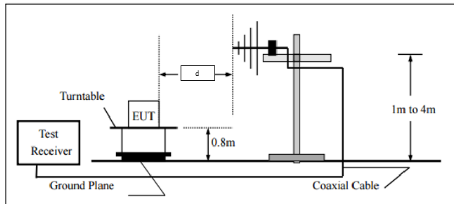
Fig. 21: Radio-frequency radiated emissions of table top equipment from 30 MHz to 1000 MHz Distance "d" depends on test chamber.
