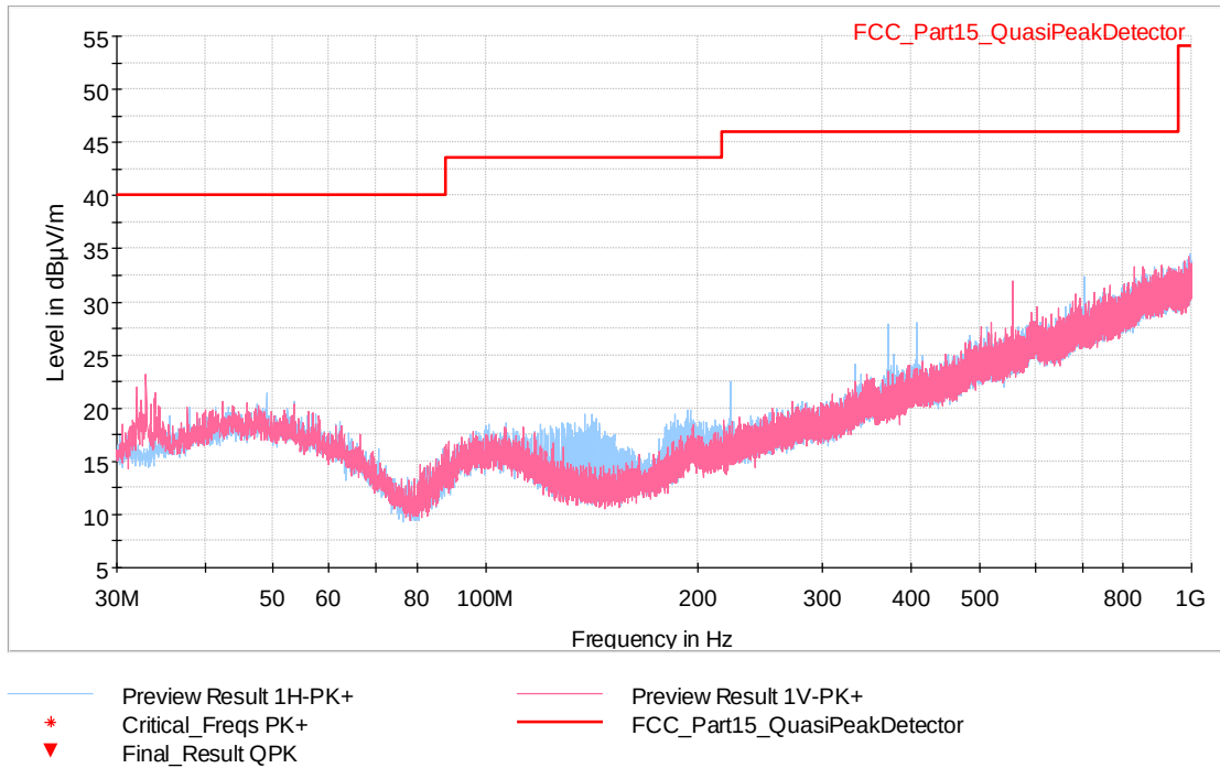
Fig. 23: Ambient level. Frequency range: 30 MHz – 1 GHz
