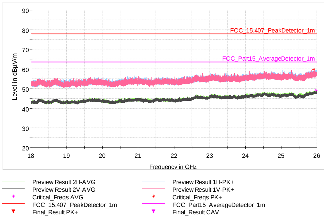
Fig. 26: Ambient level. Frequency range: 18 GHz – 26 GHz
