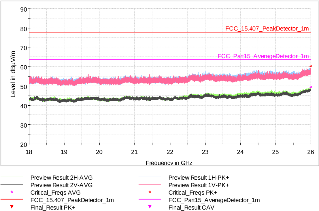
Fig. 38: Sample #1. Mode 1. Frequency range: 18 GHz – 26 GHz. Channel High
