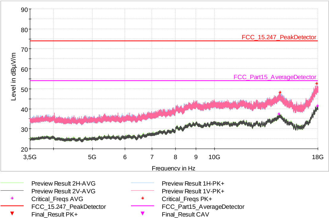
Fig. 34: Sample #1. Mode 1. Frequency range: 3.5 GHz – 18 GHz. Channel Middle
