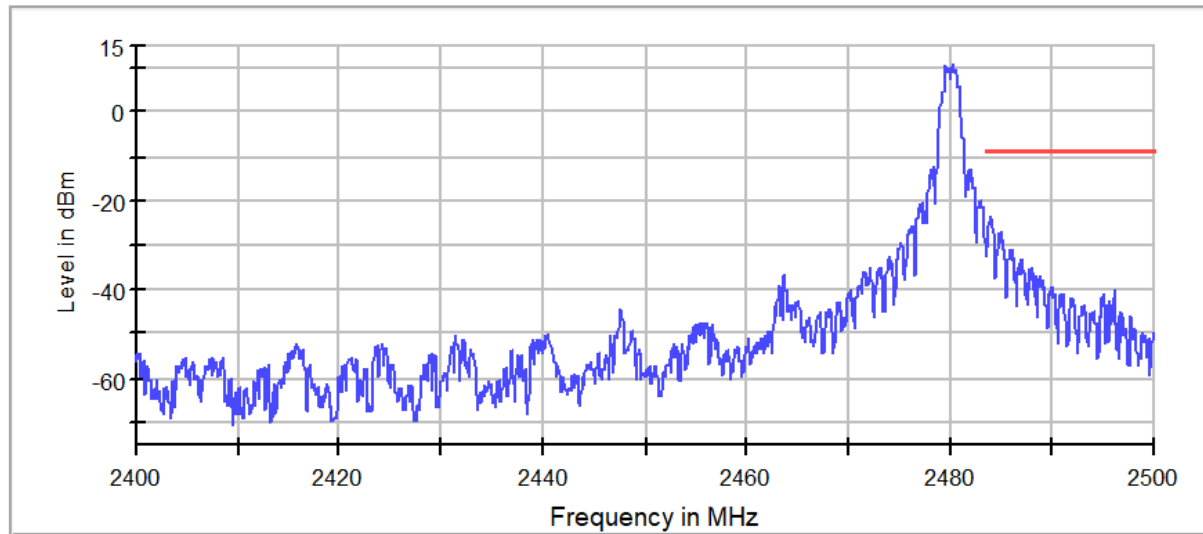
Fig. 19: Channel High - Band Edge
