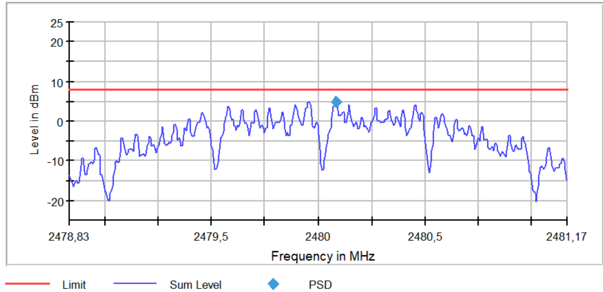
Fig. 16: Channel High- Power Spectral Density
