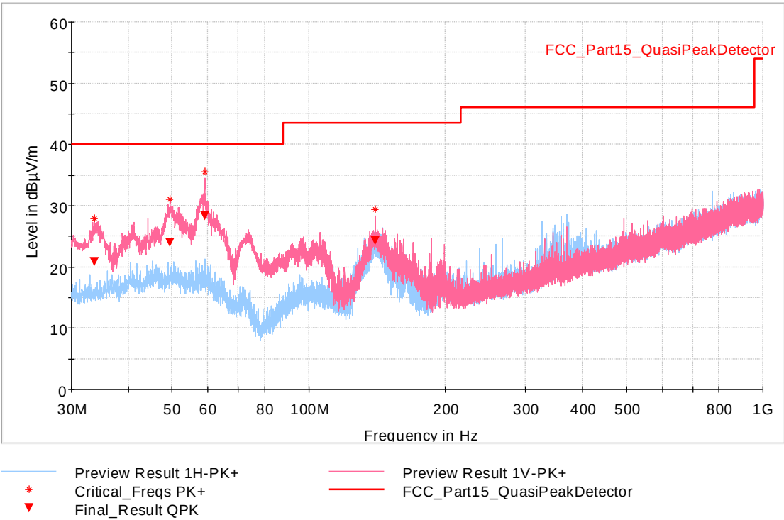
Fig. 27: Sample #1. Mode 1. Frequency range: 30 MHz – 1 GHz. Channel Low
