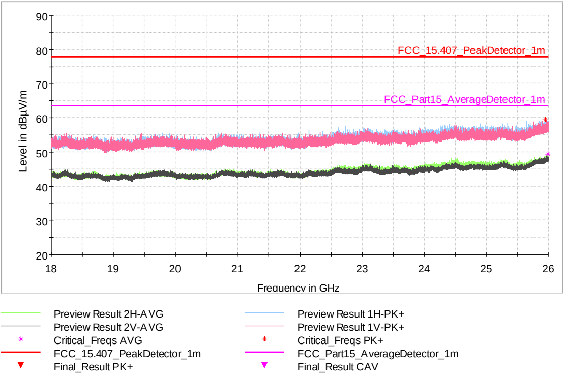
Fig. 36: Sample #1. Mode 1. Frequency range: 18 GHz – 26 GHz. Channel Low
