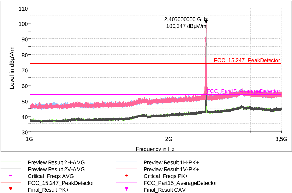
Fig. 30: Sample #1. Mode 1. Frequency range: 1 GHz – 3.5 GHz. Channel Low
