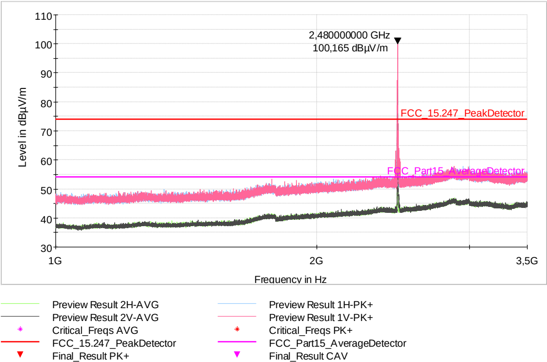
Fig. 32: Sample #1. Mode 1. Frequency range: 1 GHz – 3.5 GHz. Channel High
