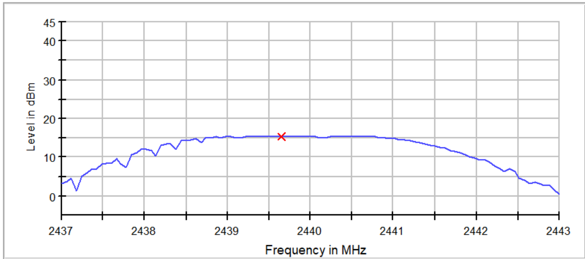
Fig. 11: Channel Middle - Maximum Peak Conducted Output Power
