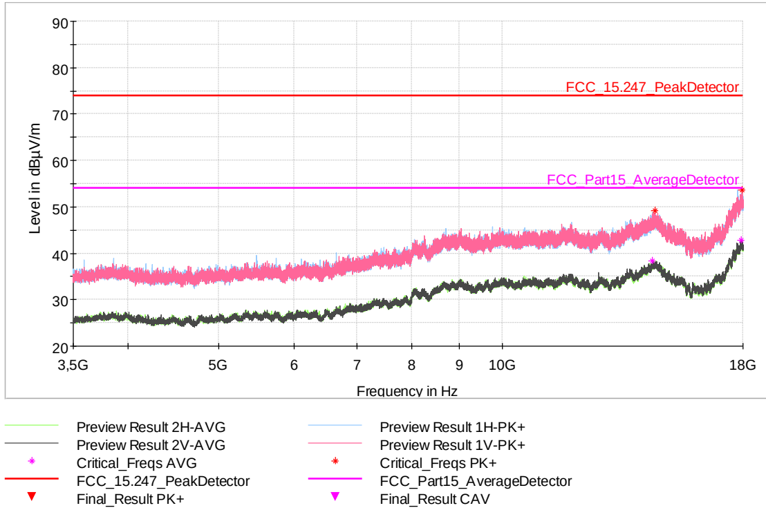
Fig. 25: Ambient level. Frequency range: 3.5 GHz – 18 GHz
