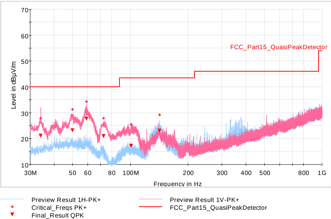
Fig. 29: Sample #1. Mode 1. Frequency range: 30 MHz – 1 GHz. Channel High
