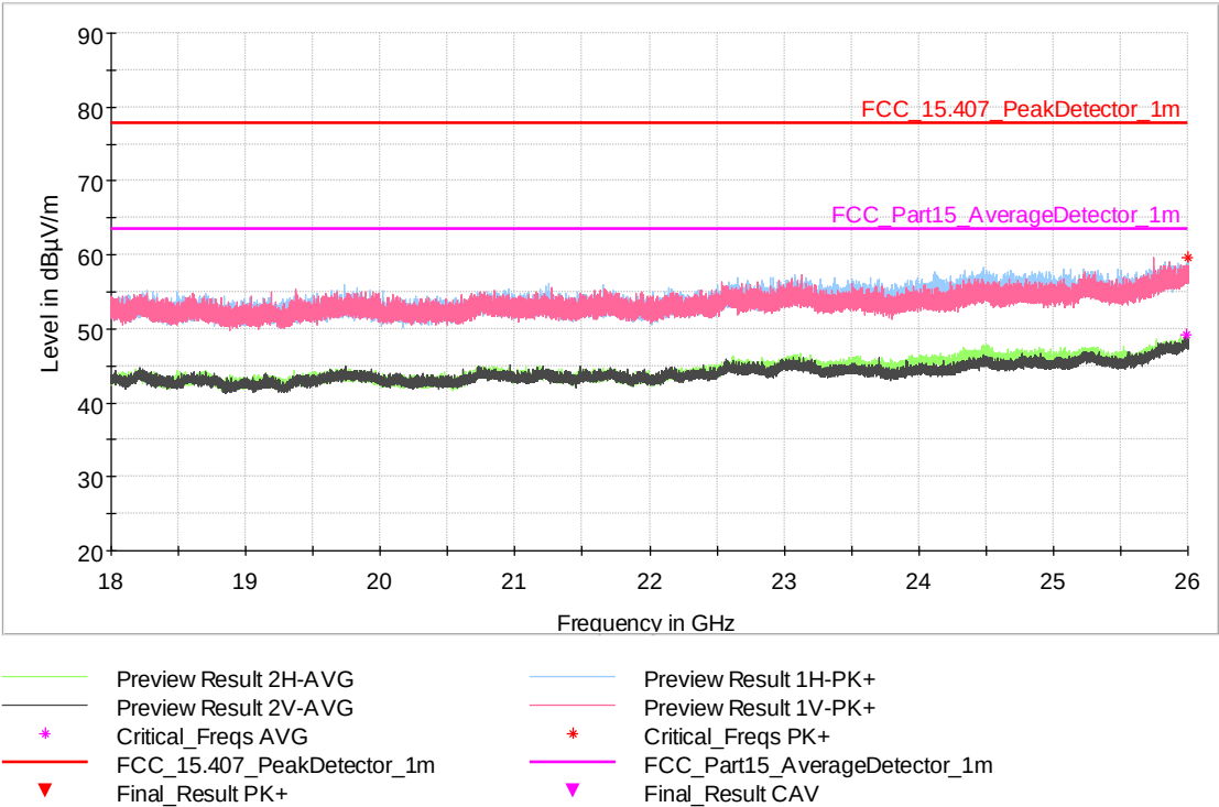
Fig. 37: Sample #1. Mode 1. Frequency range: 18 GHz – 26 GHz. Channel Middle
