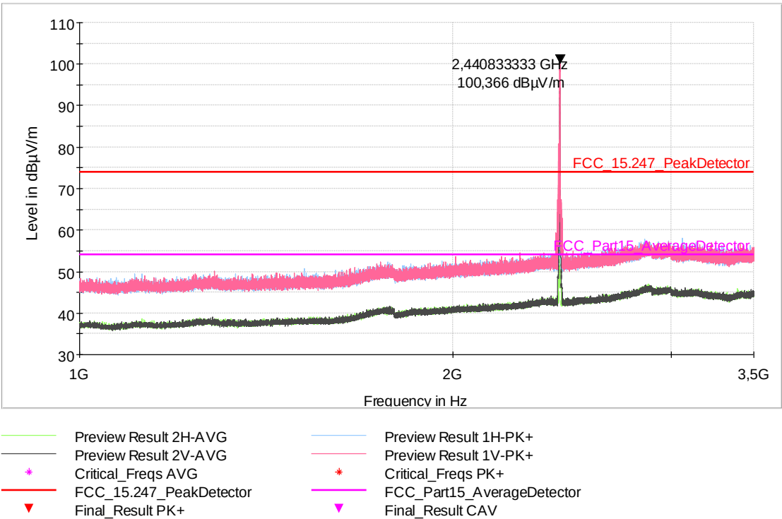
Fig. 31: Sample #1. Mode 1. Frequency range: 1 GHz – 3.5 GHz. Channel Middle
