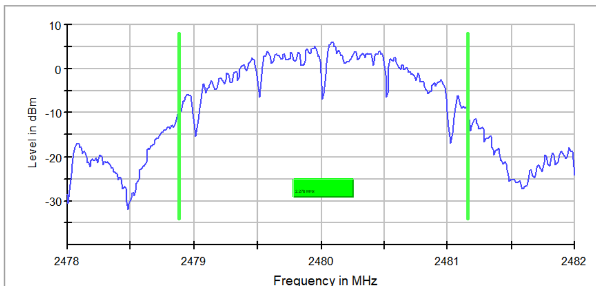
Fig. 4: Channel High 99% Occupied Channel Bandwidth
