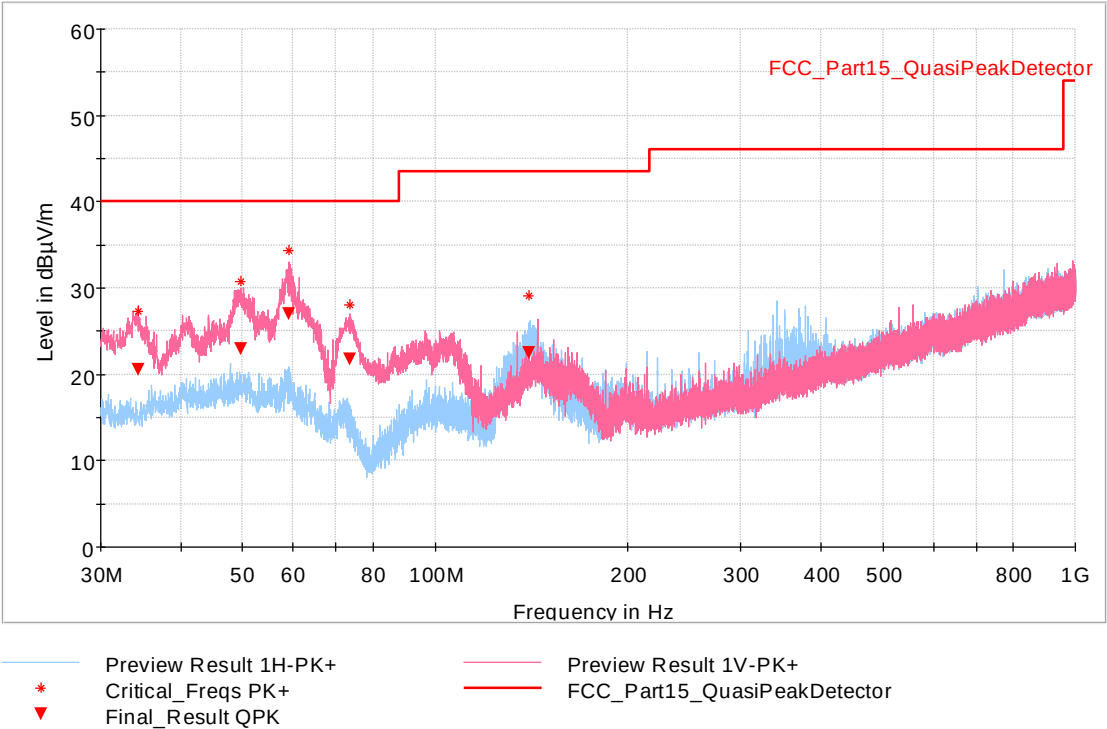
Fig. 28: Sample #1. Mode 1. Frequency range: 30 MHz – 1 GHz. Channel Middle
