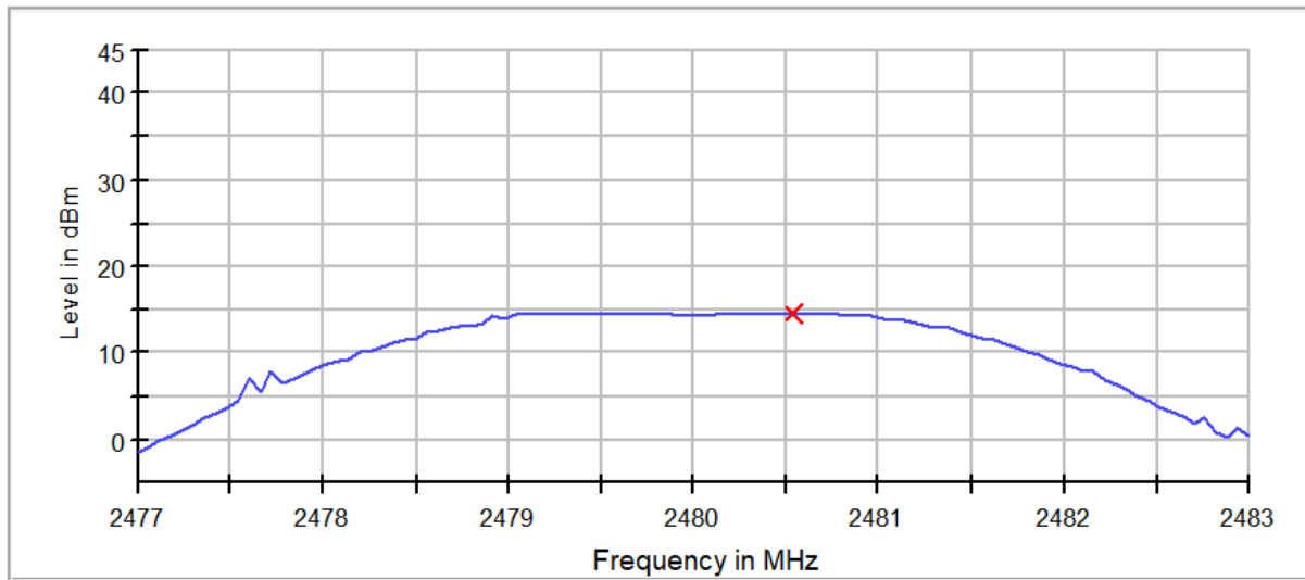
Fig. 12: Channel High - Maximum Peak Conducted Output Power
