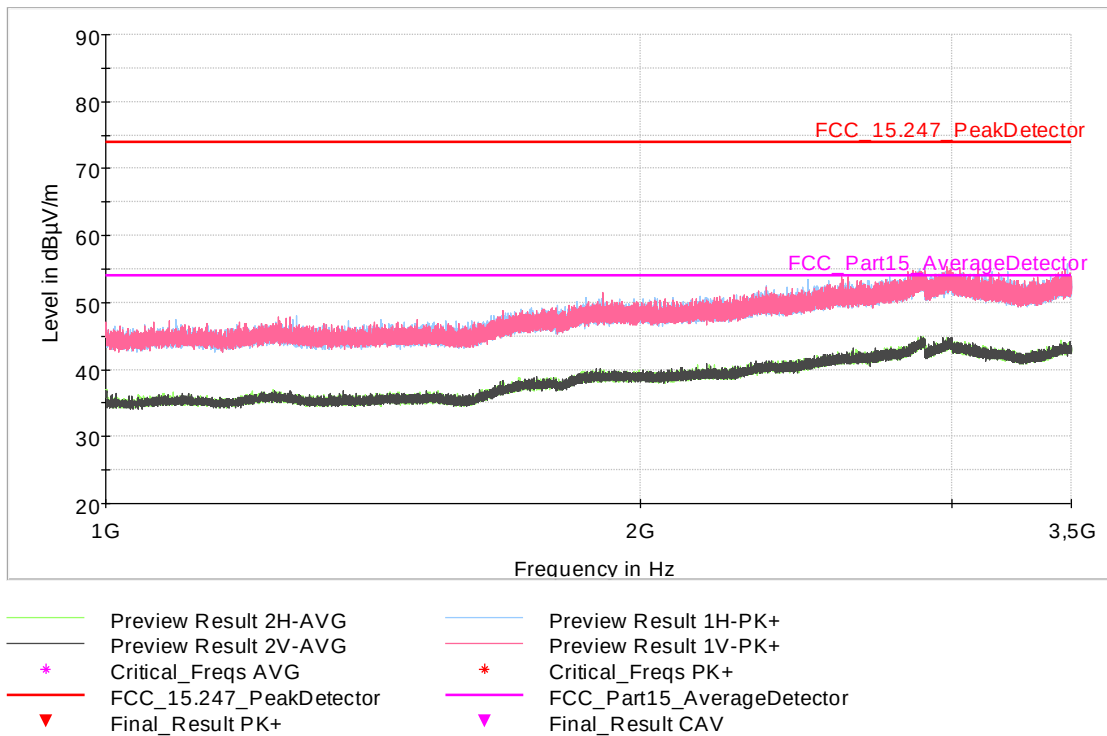
Fig. 24: Ambient level. Frequency range: 1 GHz – 3.5 GHz
