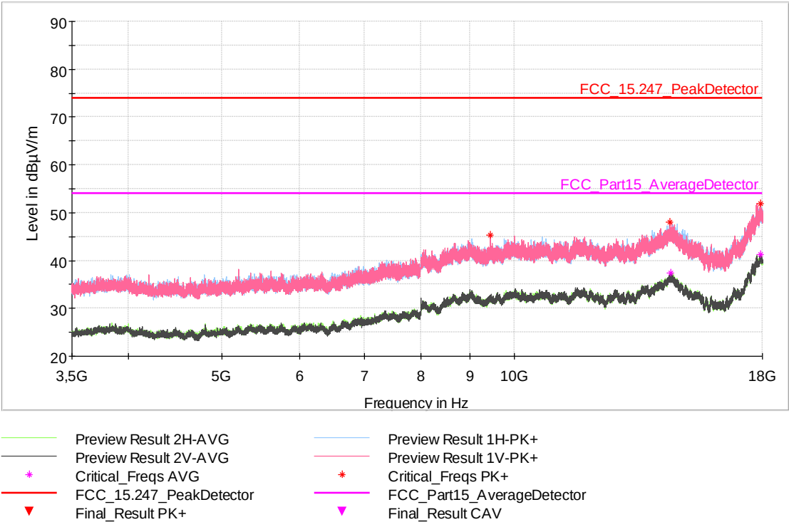
Fig. 35: Sample #1. Mode 1. Frequency range: 3.5 GHz – 18 GHz. Channel High
