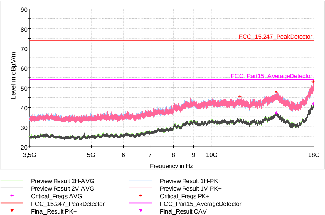
Fig. 33: Sample #1. Mode 1. Frequency range: 3.5 GHz – 18 GHz. Channel Low
