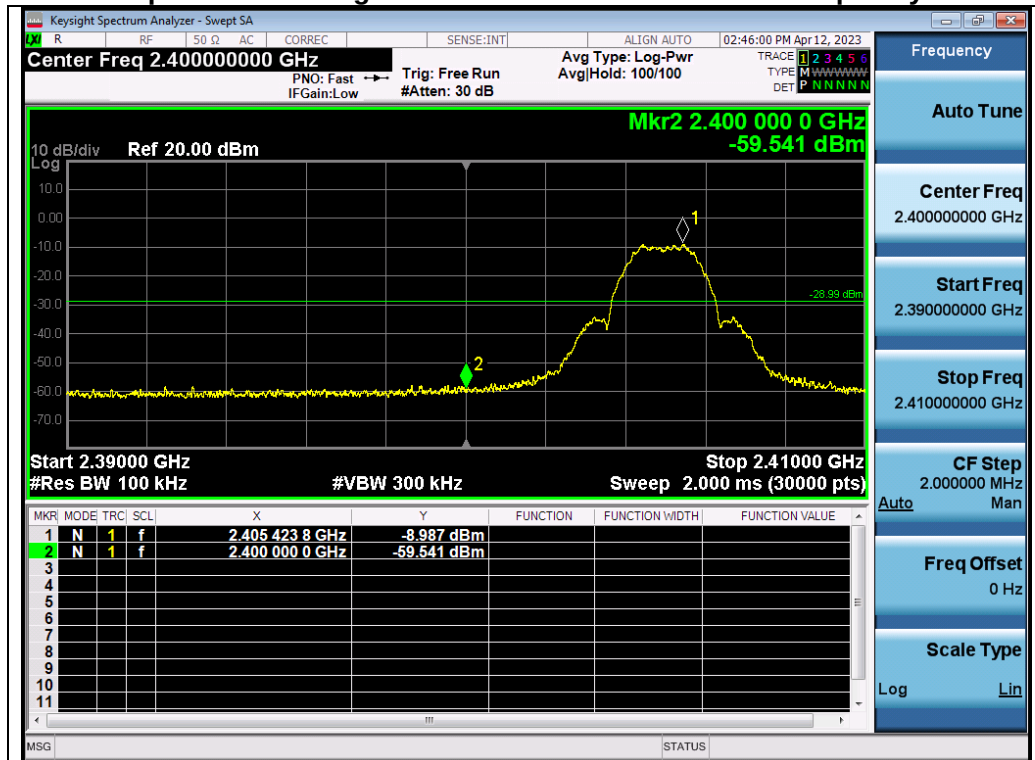
Test_Graph_2.4G_ANT1_2405_2Mbps_Lower Band Edge Emissions
