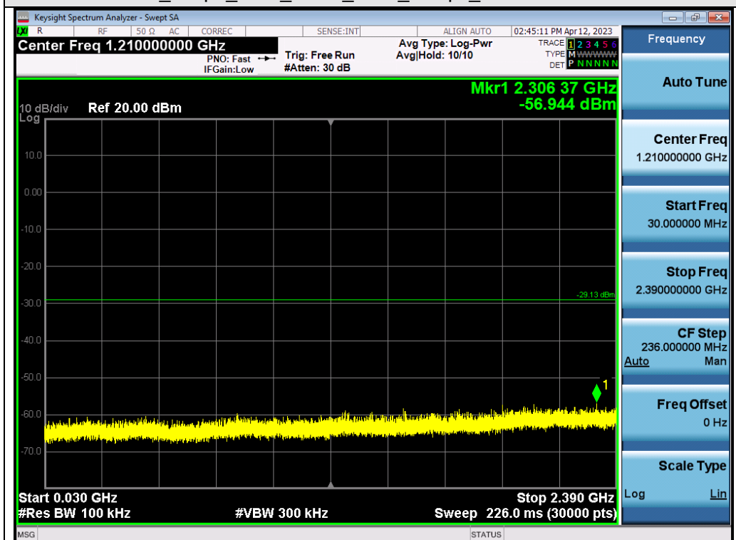
Test_Graph_2.4G_ANT1_2405_2Mbps_Lower Band Emissions
