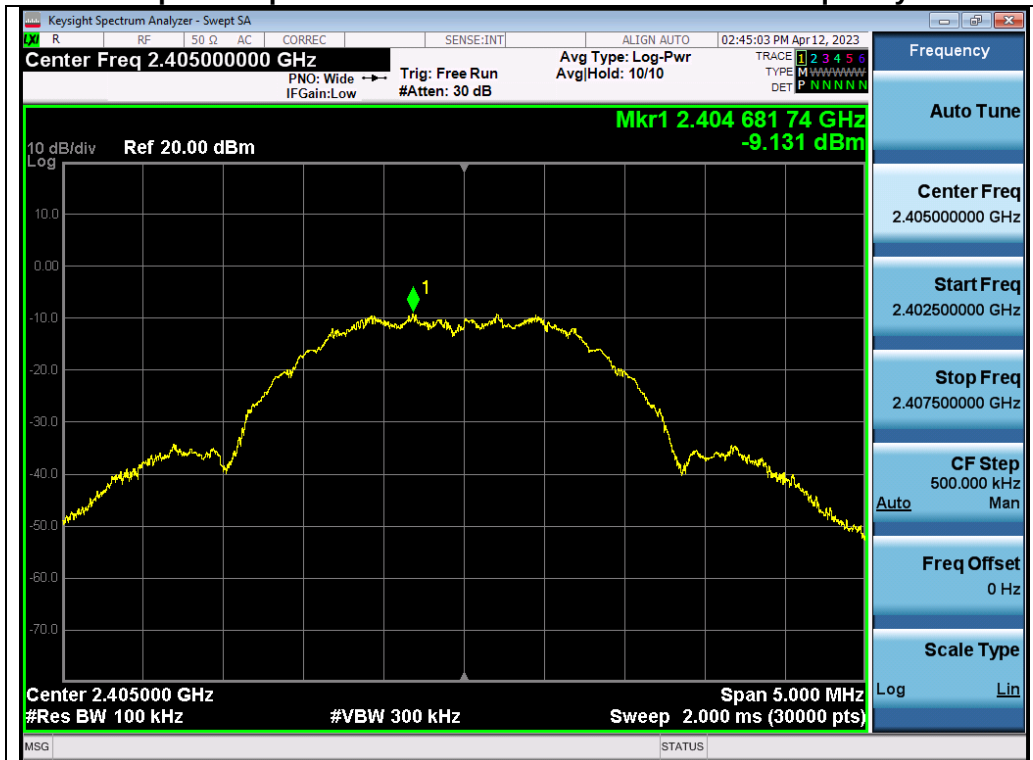
Test_Graph_2.4G_ANT1_2405_2Mbps_Reference Level
