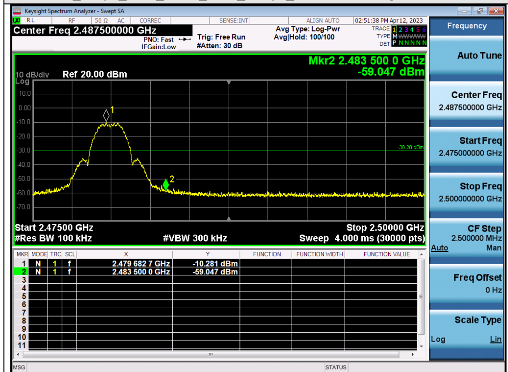
Test_Graph_2.4G_ANT1_2480_2Mbps_Higher Band Edge Emissions
