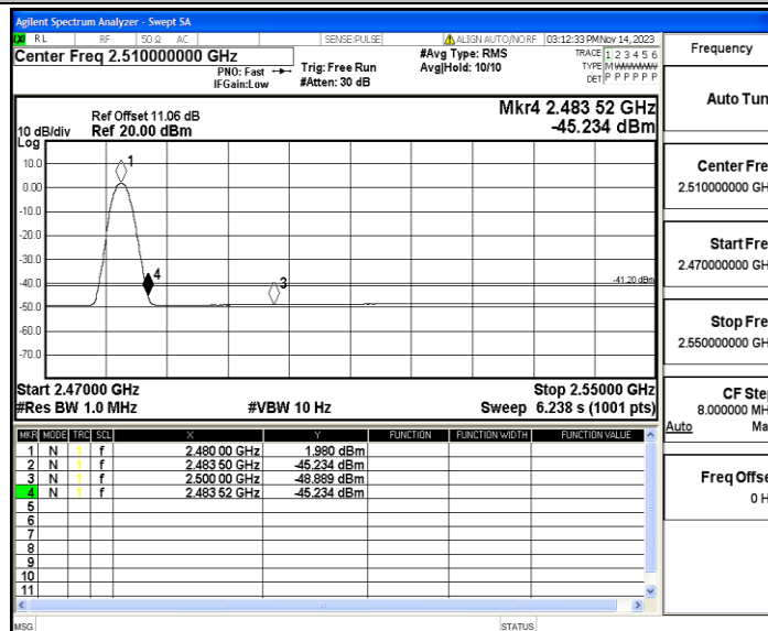
SRD_Ant1_High_2480_Peak
