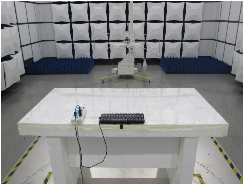
Radiated Emission Below 1GHz(worst case: with adapter)
