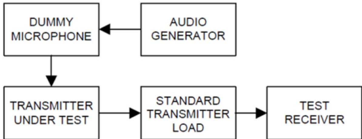
Figure 7.9.1 Audio frequency response test test setup
