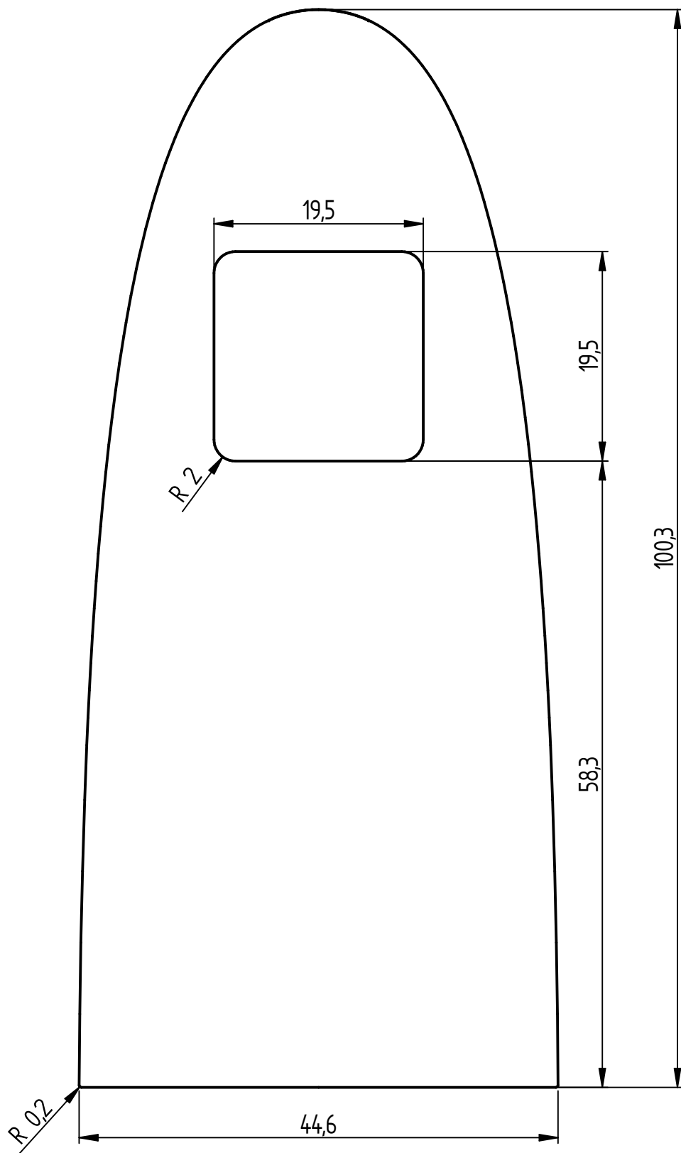
Mechanical Part
