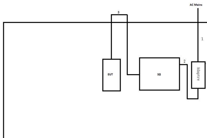
Test Setup Diagram - Radiated Test (USB mode; TX)
