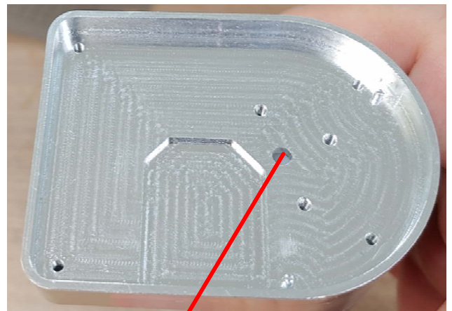
Waveguide for radar signal coupling
