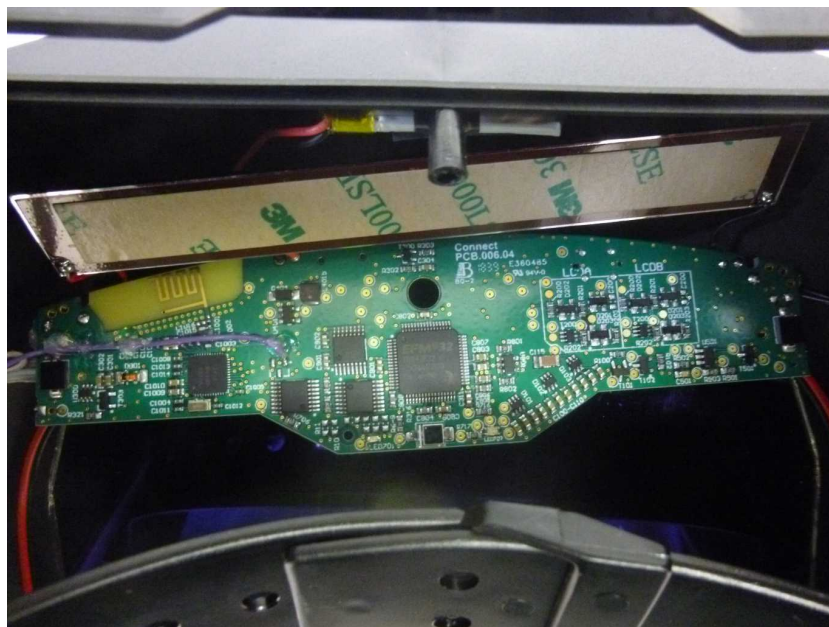
Photo 2: PCB back side view, inside the helmet
