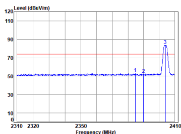
BLE_2M_TX_CH_01_Horizontal-Peak
