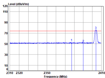
BLE_2M_TX_CH_01_Vertical-Peak
