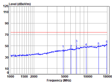
BLE_2M_TX_CH_01_Horizontal-Peak
