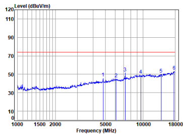
BLE_2M_TX_CH_01_Vertical-Peak
