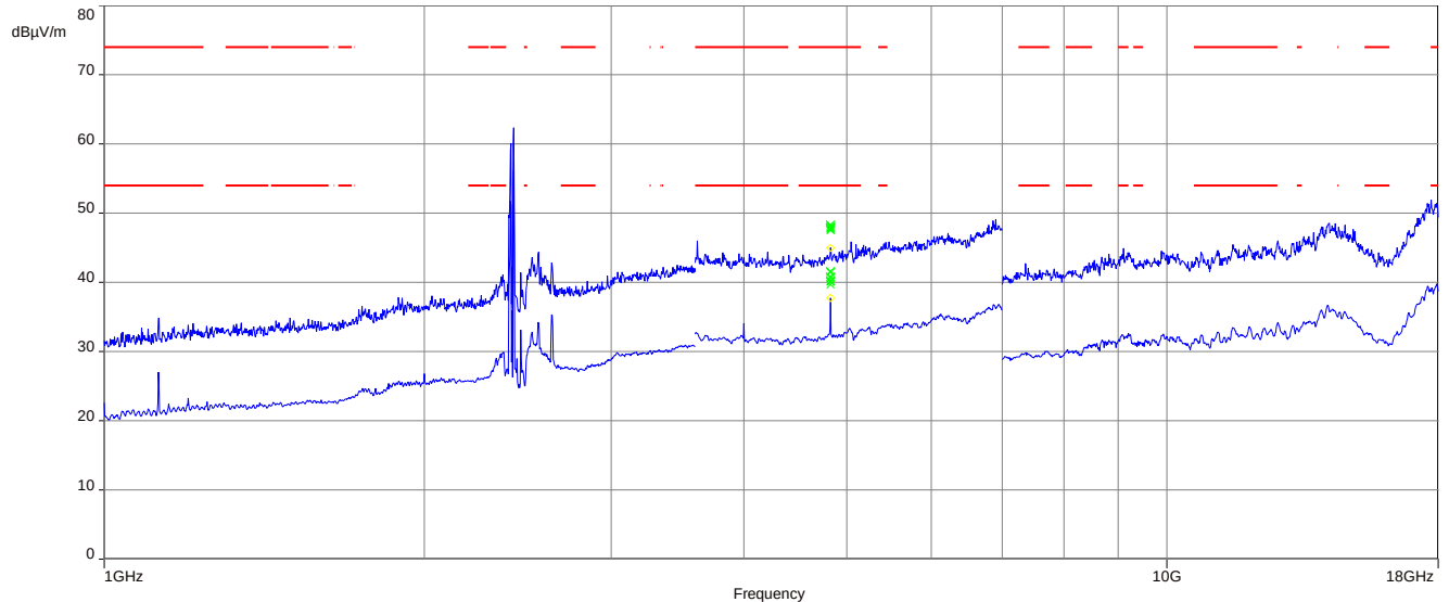
Plot 1: Lowest channel, 1 GHz to 18 GHz, vertical & horizontal polarization
