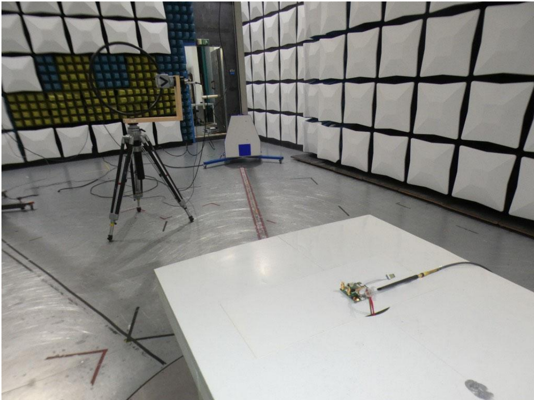
Photo 1: Test setup for H-Field measurements
