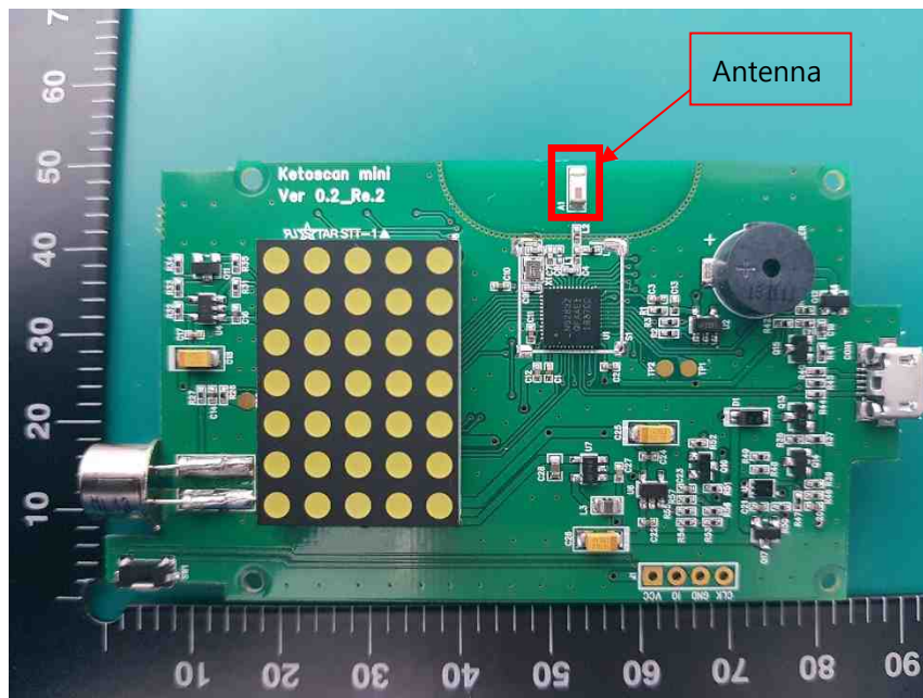
Main board - Front Top (Remove shield can)
