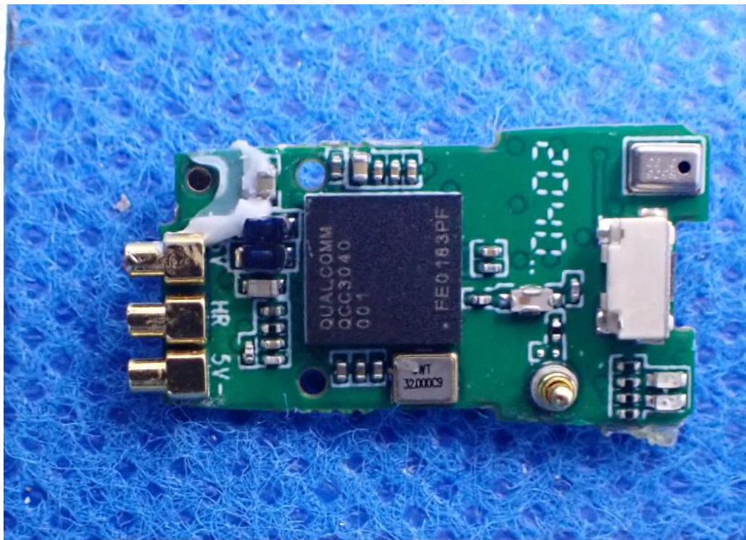
Right VIEW OF EUT(PORT)
