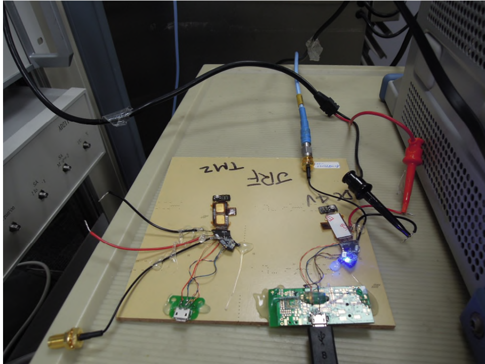
Photograph 15: Set-up for Conducted testing – Right Ear
