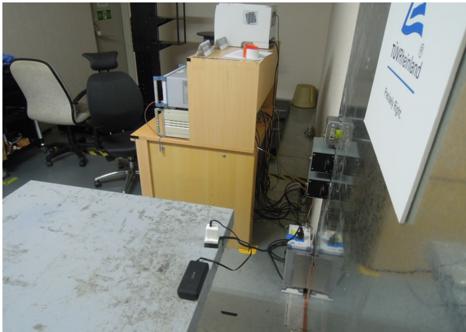
Photograph 16: Set-up for Mains Conducted testing (Back View)
