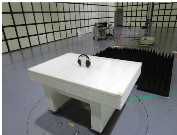
Above 1 GHz
