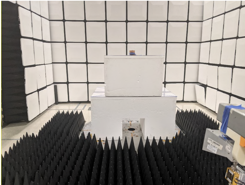
Figure 4 - Radiated emissions above 1 GHz, front view
