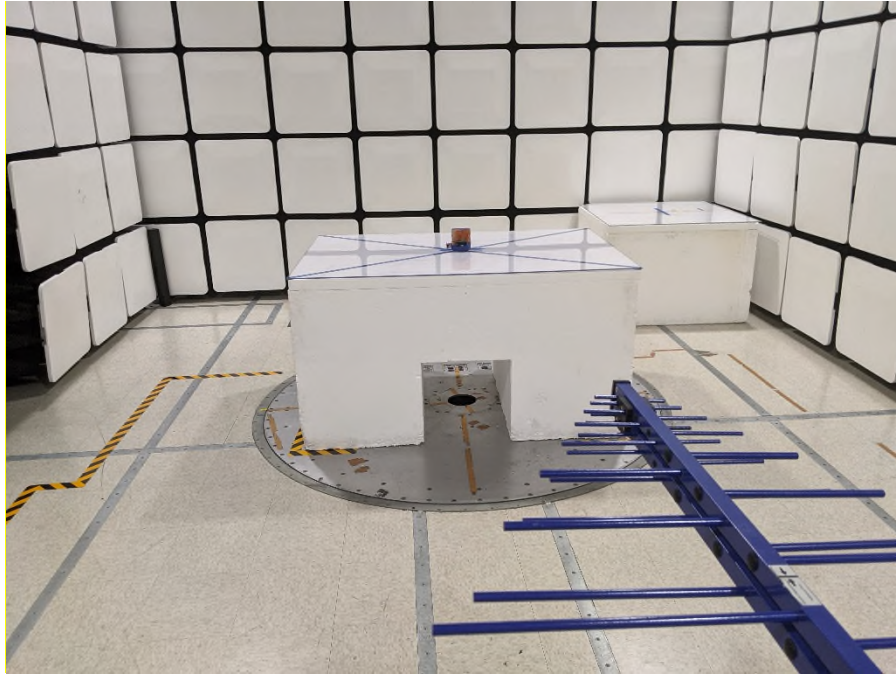
Figure 2 - Radiated emissions below 1 GHz, front view
