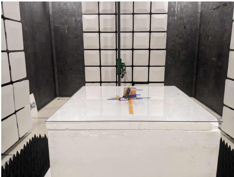
Figure 5 - Radiated emissions above 1 GHz, back view
