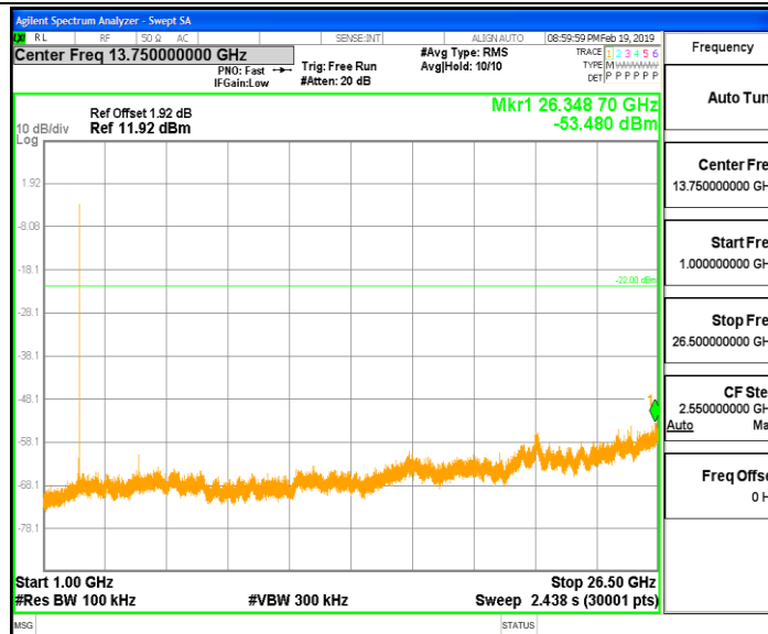
3DH1_Ant1_2402_0~Reference
