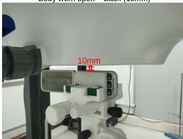
Body worn open – Right (10mm)
