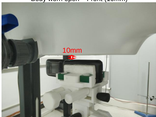
Body worn open – Left (10mm)
