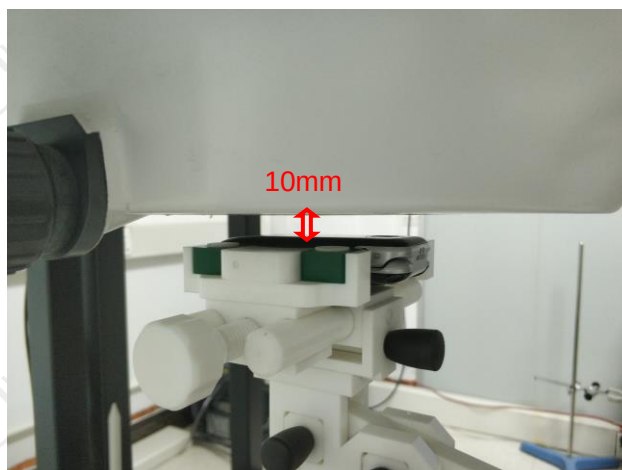
Body worn close – Back (10mm)
