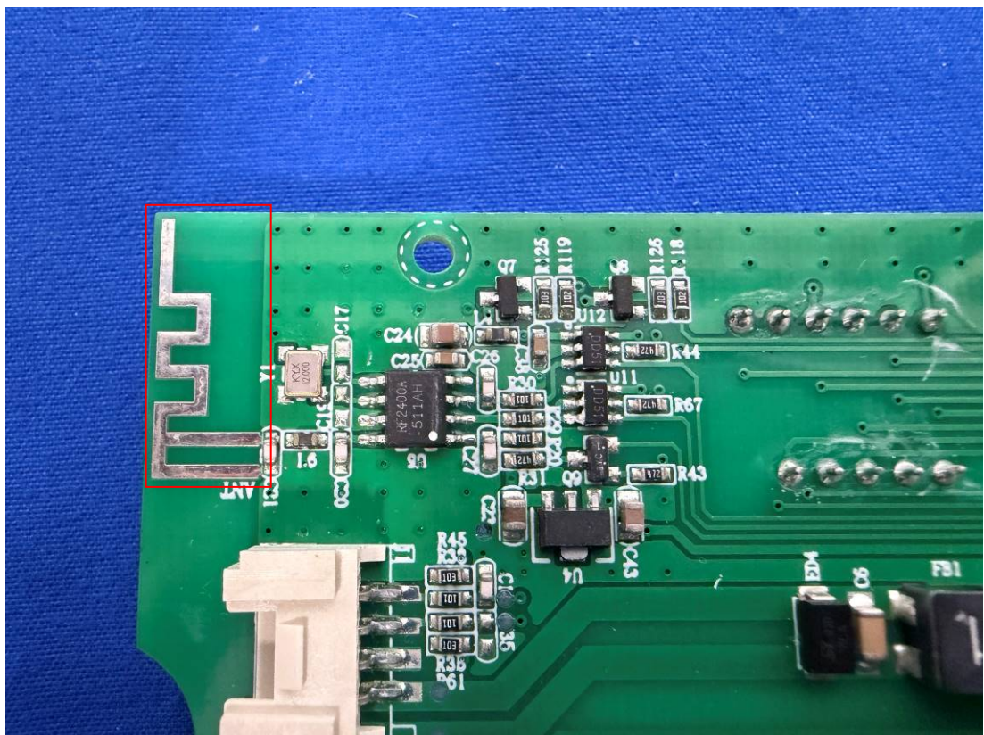
2.4G SRD Antenna(RX)
