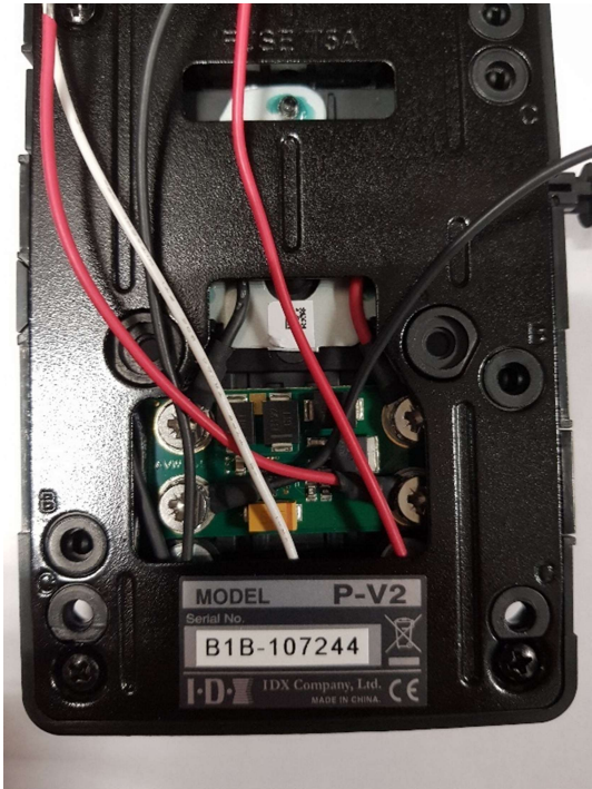
AVW0159 GALERNO Battery Limiter Board integrated
