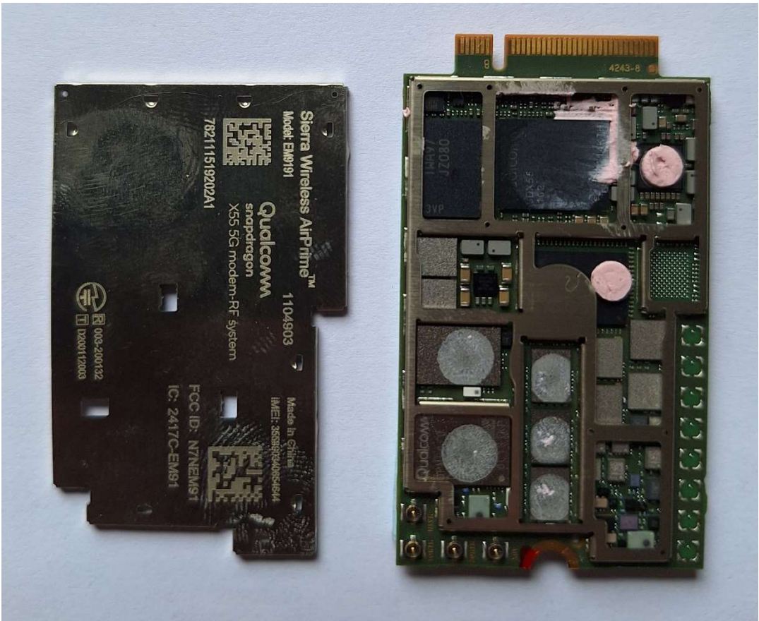
Cellular Modem
