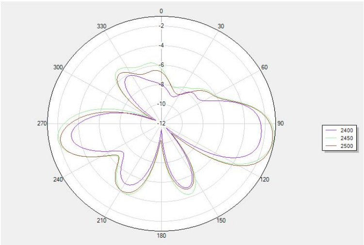
Phi 90 2D
