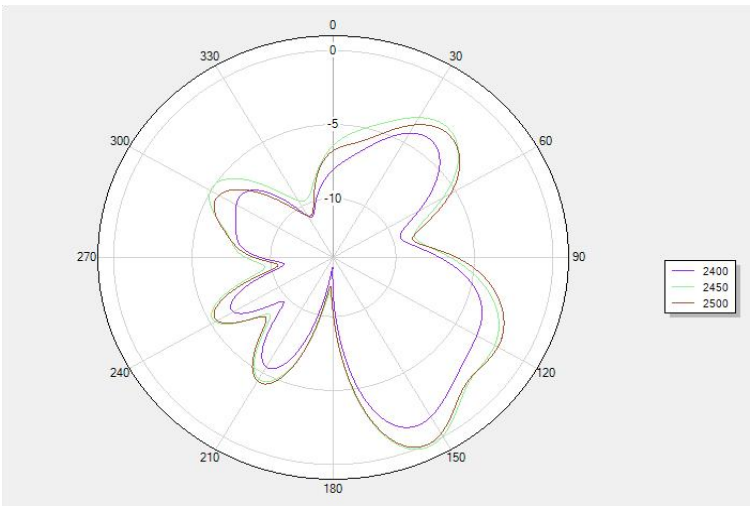
Theta 90 2D
