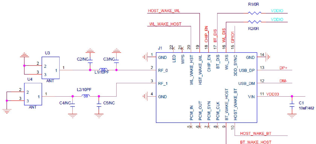
RF reference circuit
