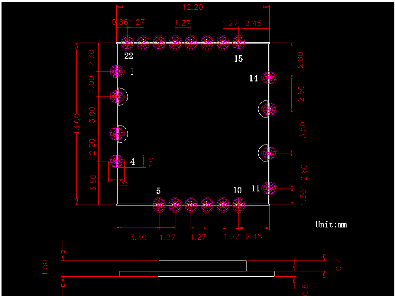
Figure 6 Module dimension
