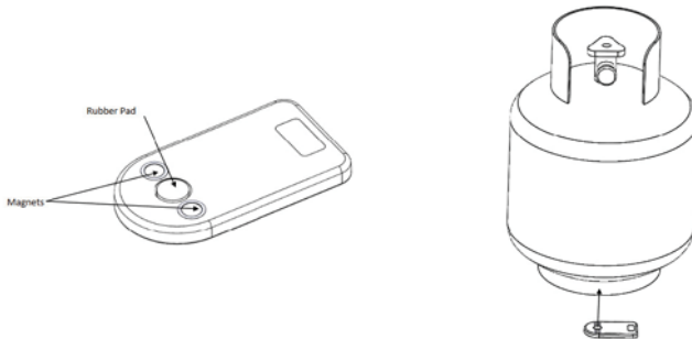
Installing SmartSense Sensors
