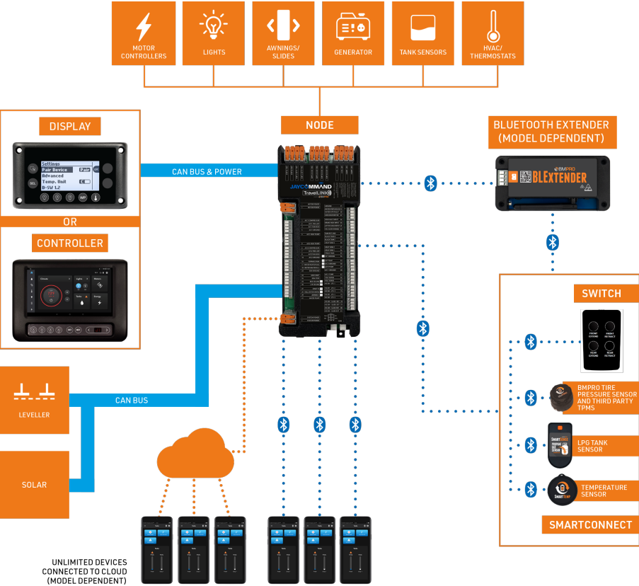
FIGURE 1: System Diagram
